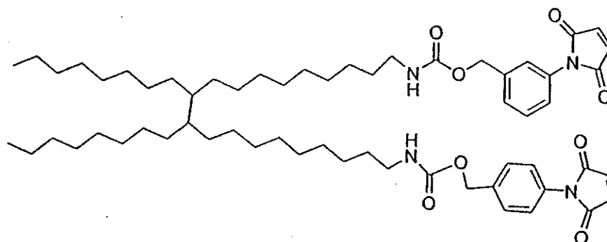
"Bis( m -maleimidobenzyl carbamate) of DDI 1410" (and cyclic isomers)
