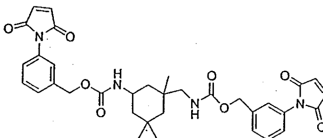
"Bis( m -maleimidobenzyl carbamate) of IPDI"
