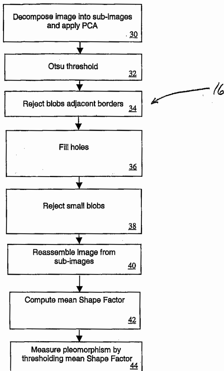
Figure 2 Nuclear Pleomorphism Feature Detection
