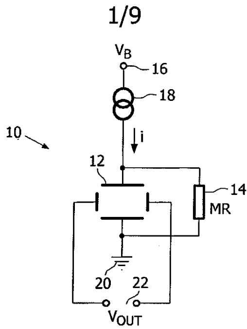
FIG. 1 PRIOR ART
