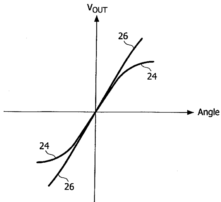
FIG. 2 PRIOR ART
