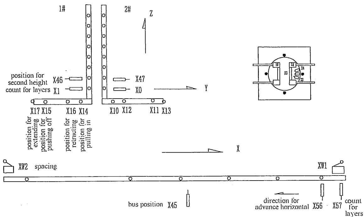
layout diagram of sensors on merchenical arms (47 points)
