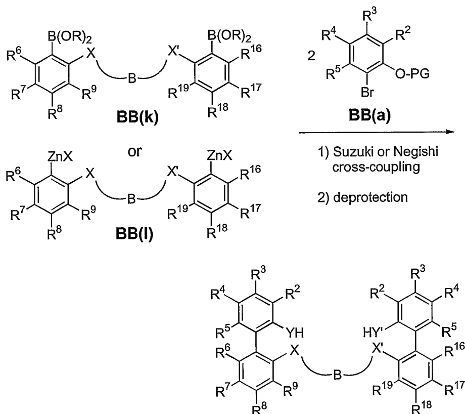
Scheme 14
