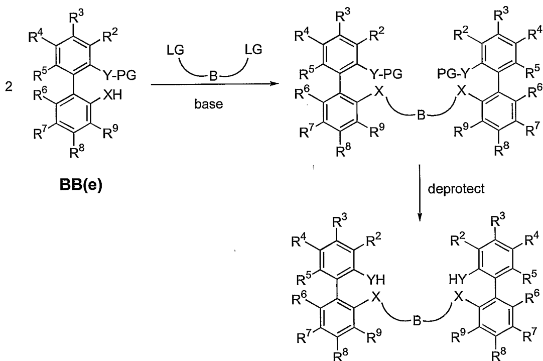
Scheme 9
