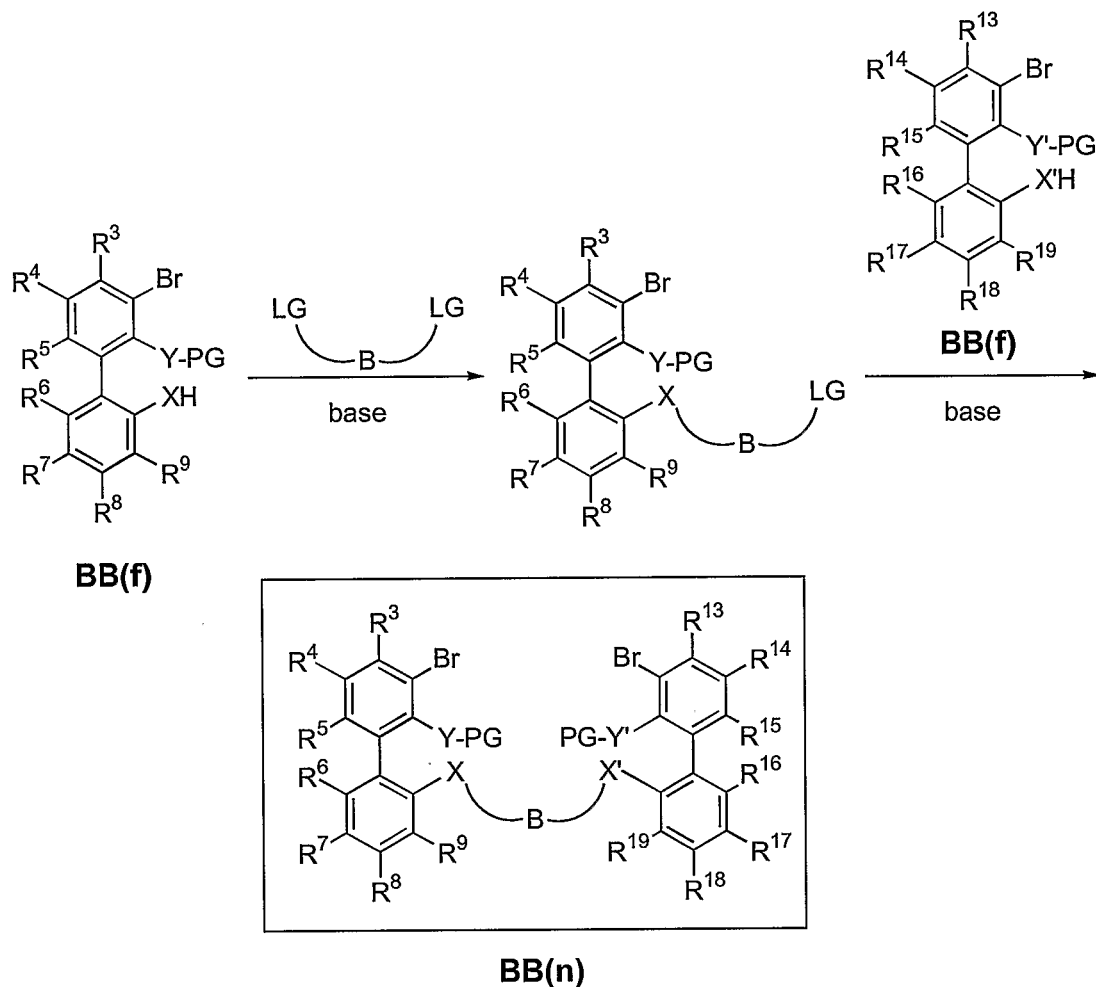
Scheme 8
