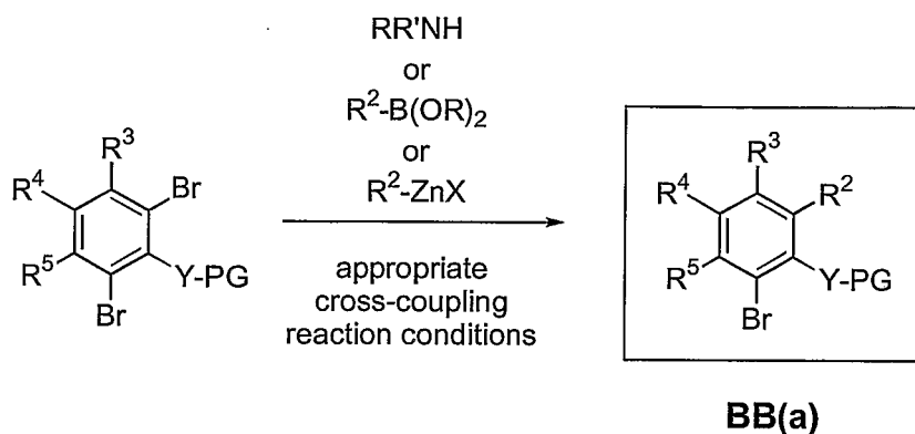
Scheme 1b
