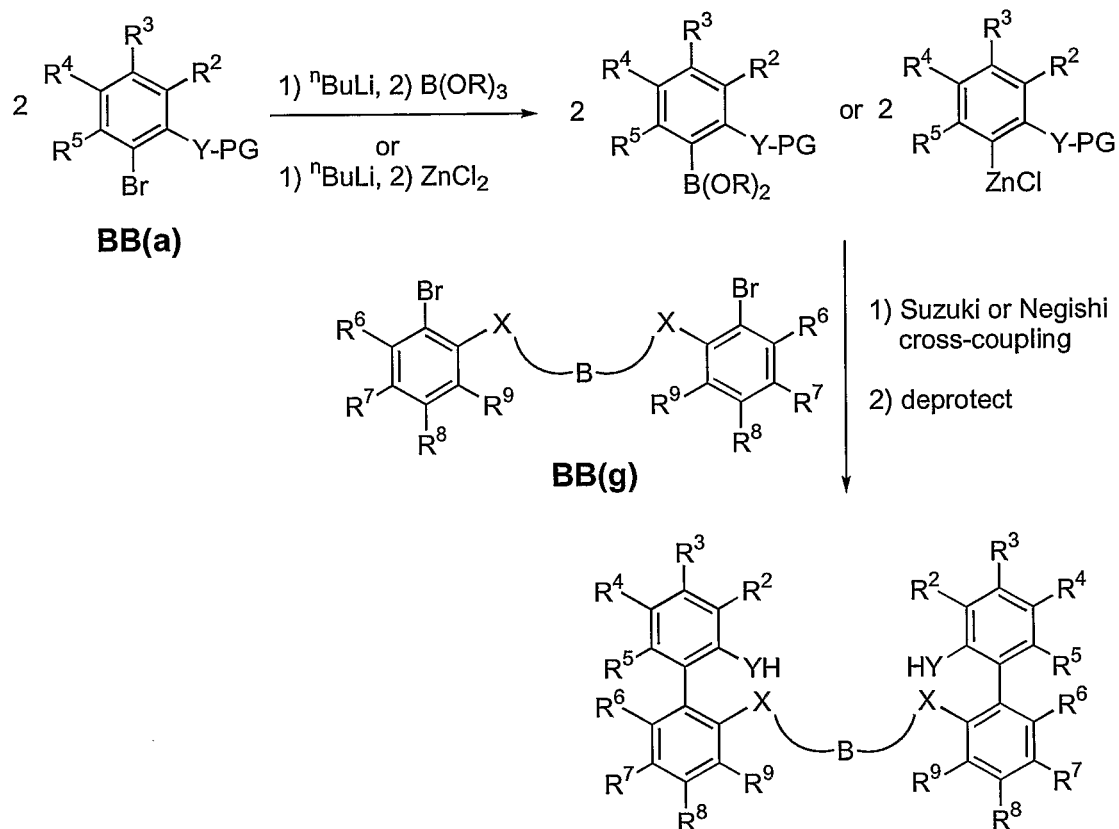
Scheme 11
