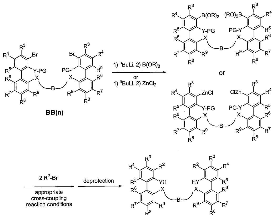
Scheme 17
