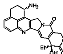
DX8951f
