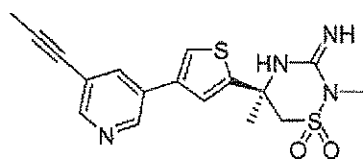
Example 47
