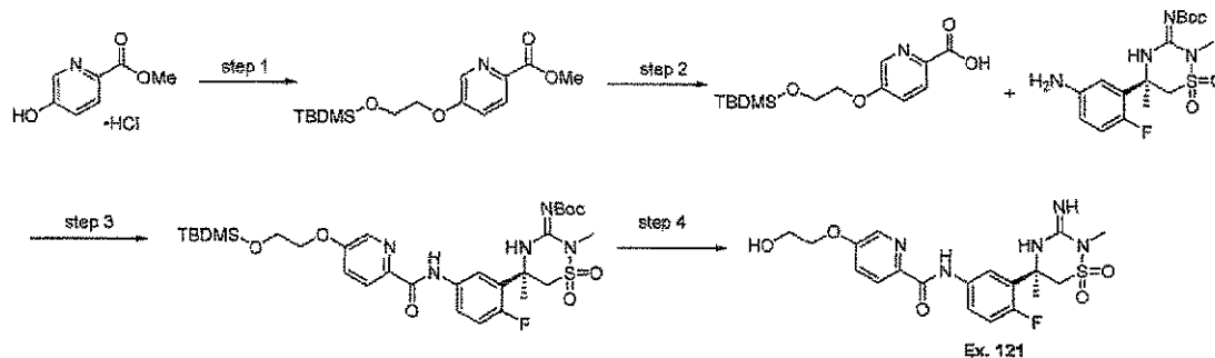
Scheme 24:
