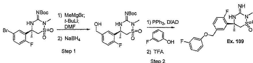
Scheme 21:
