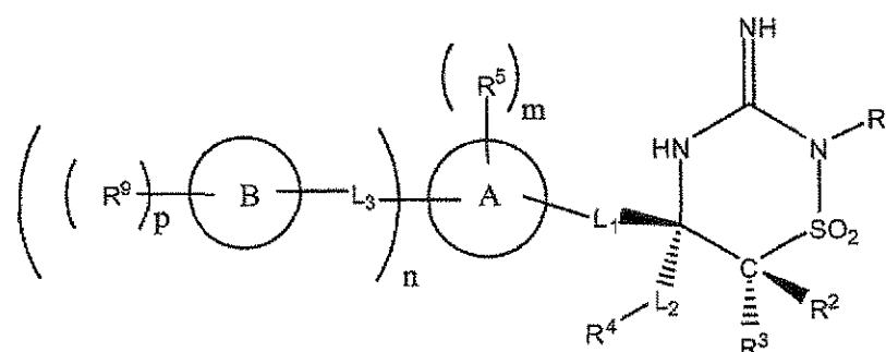
(IA-2)
