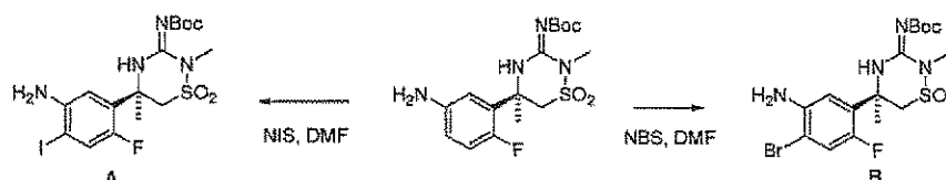
Scheme 10a:
