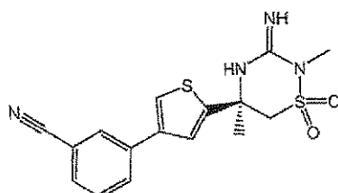
Example 45
