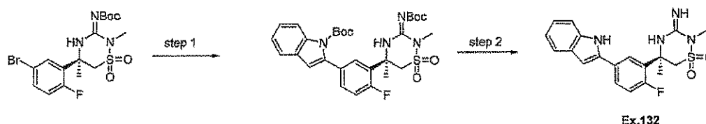
Scheme 30:
