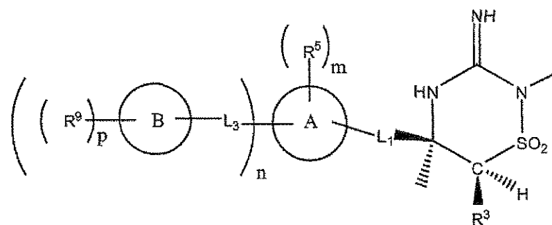
(IIA-1)
