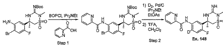
Scheme 34:
