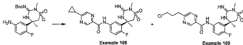
Scheme 41:
