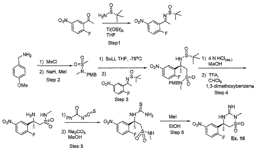
Scheme 3a:
