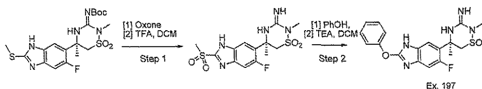
Scheme 51:
