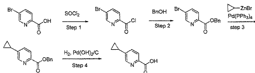
Scheme 11u:
