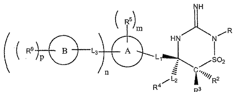
(IA-1)
