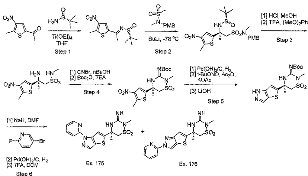
Scheme 44:
