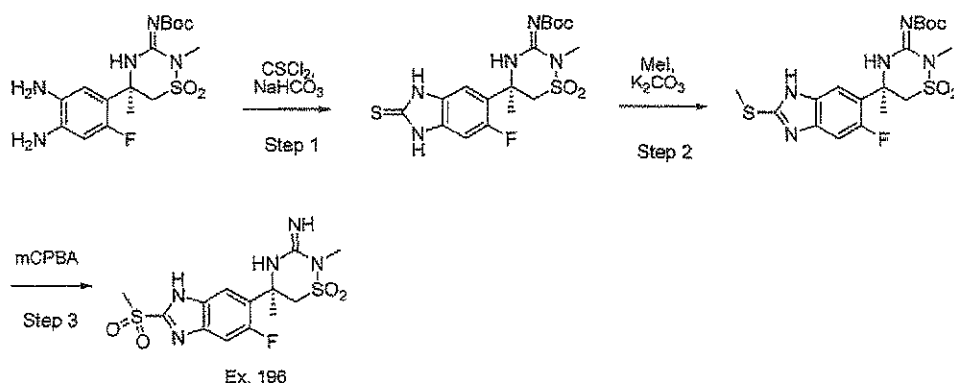
Scheme 50:
