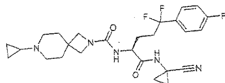
N-[(S)-1-(1-cyanocyclopropylcarbamoyl)-4,4-difluoro-4-(2-fluorophenyl)butyl]-7-cyclopropyl-2,7-diazaspiro[3.5]nonane-2-carboxamide
