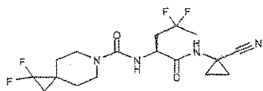
N-[(S)-1-(1-cyanocyclopropylcarbamoyl)-3,3-difluoropentyl]-1,1-difluoro-6-azaspiro[2.5]octane-6-carboxamide
