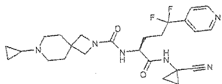
10 N-[(S)-1-(1-cyanocyclopropylcarbamoyl)-3,3-difluoro-4-phenylbutyl]-7-methyl-2,7-diazaspiro[3.5]nonane-2-carboxamide
