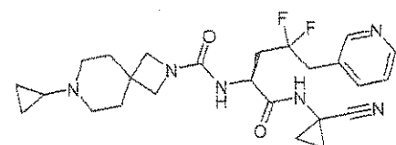
15 N-[(S)-1-(1-cyanocyclopropylcarbamoyl)-3,3-difluoro-4-pyridin-4-ylbutyl]- 7-cyclopropyl-2,7-diazaspiro[3.5]nonane-2-carboxamide
