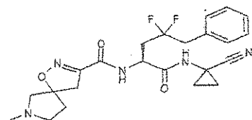
N-[(S)-1-(1-cyanocyclopropylcarbamoyl)-3,3-difluoro-4-phenylbutyl]-7-methyl-1-oxa-2,7-diazaspiro[4.4]non-2-ene-3-carboxamide
