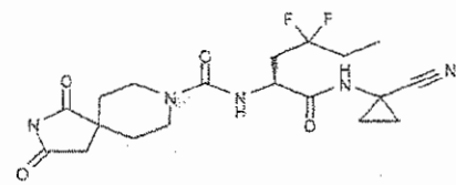
N-[(S)-1-(1-cyanocyclopropylcarbamoyl)-3,3-difluoropentyl]-1,3-dioxo-2,8-diazaspiro[4.5]decane-8-carboxamide
