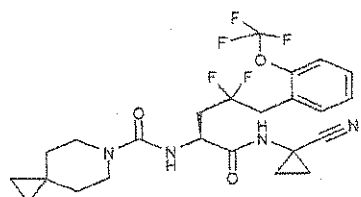
N-[(S)-1-(1-cyanocyclopropylcarbamoyl)-3,3-difluoro-4-(2-fluorophenyl)butyl]-6-azaspiro[2.5]octane-6-carboxamide
