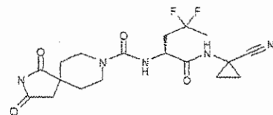
15 N-[(S)-1-(1-cyanocyclopropylcarbamoyl)-3,3-difluoro-4-phenylbutyl]-1,3-dioxo-2,8-diazaspiro[4.5]decane-8-carboxamide
