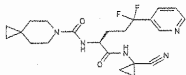
5 N-[(S)-1-(1-cyanocyclopropylcarbamoyl)-4,4-difluoro-4-pyridin-4-ylbutyl]-6-azaspiro[2.5]octane-6-carboxamide
