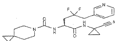
15 N-[(S)-1-(1-cyanocyclopropylcarbamoyl)-3,3-difluoro-4-pyridin-4-ylbutyl]-6-azaspiro[2.5]octane-6-carboxamide
