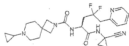
10 N-[(S)-1-(1-cyanocyclopropylcarbamoyl)-3,3-difluoro-4-pyridin-3-ylbutyl]- 7-cyclopropyl-2,7-diazaspiro[3.5]nonane-2-carboxamide
