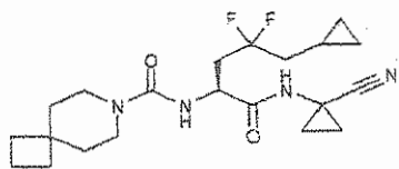
N-[(S)-1-(1-cyanocyclopropylcarbamoyl)-3,3-difluoro-4-phenylbutyl]-7-azaspiro[3.5]nonane-7-carboxamide
