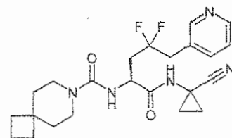
10 N-[(S)-1-(1-cyanocyclopropylcarbamoyl)-3,3-difluoro-4-pyridin-4-ylbutyl]-7-azaspiro[3.5]nonane-7-carboxamide
