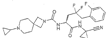
5 N-[(S)-1-(1-cyanocyclopropylcarbamoyl)-3,3-difluoro-4-(4-fluorophenyl)butyl]- 7-cyclopropyl-2,7-diazaspiro[3.5]nonane-2-carboxamide
