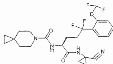
10 N-[(S)-1-(1-cyanocyclopropylcarbamoyl)-4,4-difluoro-4-(4-fluorophenyl)butyl]-6-azaspiro[2.5]octane-6-carboxamide
