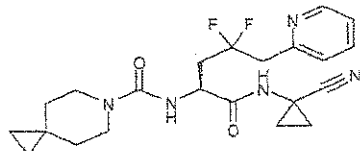
10 N-[(S)-1-(1-cyanocyclopropylcarbamoyl)-3,3-difluoro-4-pyridin-3-ylbutyl]-6-azaspiro[2.5]octane-6-carboxamide
