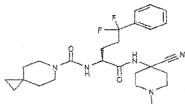
5 N-[(S)-1-(1-cyanocyclopropylcarbamoyl)-4,4-difluoro-4-phenylbutyl]-7-cyclopropyl-2,7-diazaspiro[3.5]nonane-2-carboxamide
