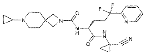
5 N-[(S)-1-(1-cyanocyclopropylcarbamoyl)-4,4-difluoro-4-pyridin-3-ylbutyl]-7-cyclopropyl-2,7-diazaspiro[3.5]nonane-2-carboxamide
