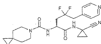
15 N-[(S)-1-(1-cyanocyclopropylcarbamoyl)-3,3-difluoro-4-pyridin-4-ylbutyl]-6-azaspiro[2.5]octane-6-carboxamide
