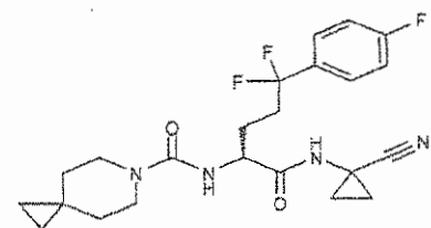
15 N-[(S)-1-(1-cyanocyclopropylcarbamoyl)-4,4-difluoro-4-(2-fluorophenyl)butyl]-6-azaspiro[2.5]octane-6-carboxamide
