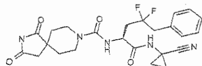
15 N-[(S)-1-(1-cyanocyclopropylcarbamoyl)-3,3-difluoro-4-phenylbutyl]-1,3-dioxo-2,8-diazaspiro[4.5]decane-8-carboxamide
