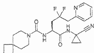
N-[(S)-1-(1-cyanocyclopropylcarbamoyl)-3,3-difluoro-4-pyridin-3-ylbutyl]-7-azaspiro[3.5]nonane-7-carboxamide
