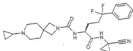
N-[(S)-1-(1-cyanocyclopropylcarbamoyl)-4,4-difluoro-4-(4-fluorophenyl)butyl]-7-cyclopropyl-2,7-diazaspiro[3.5]nonane-2-carboxamide
