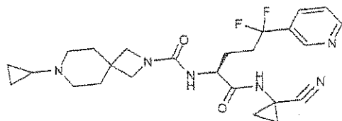
N-[(S)-1-(1-cyanocyclopropylcarbamoyl)-4,4-difluoro-4-pyridin-4-ylbutyl]-7-cyclopropyl-2,7-diazaspiro[3.5]nonane-2-carboxamide
