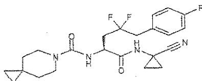
N-[(S)-1-(1-cyanocyclopropylcarbamoyl)-3,3-difluoro-4-pyridin-2-ylbutyl]-6-azaspiro[2.5]octane-6-carboxamide
