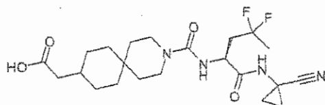
5 {3-[(S)-1-(1-cyanocyclopropylcarbamoyl)-3,3-difluoropentylcarbamoyl]-3-azaspiro[5.5]undec-9-yl}acetic acid
