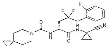
5 N-[(S)-1-(1-cyanocyclopropylcarbamoyl)-3,3-difluoro-4-(4-fluorophenyl)butyl]-6-azaspiro[2.5]octane-6-carboxamide
