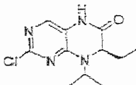
(7R)-2-chloro-7-ethyl-8-isopropyl-7,8-dihydro-5H-pteridin-6-one.
