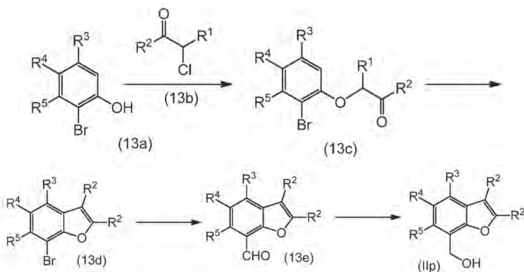
Scheme 13
