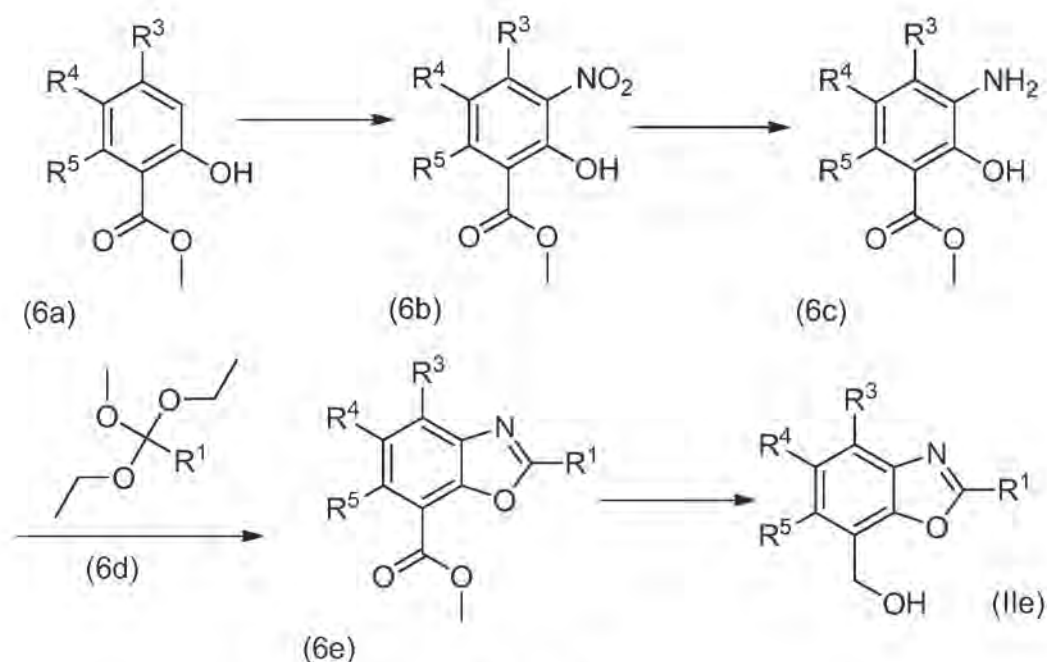
Scheme 6
