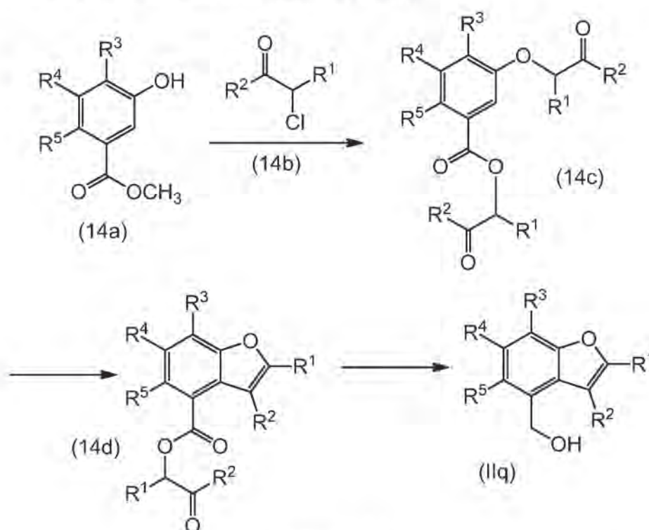
Scheme 14
