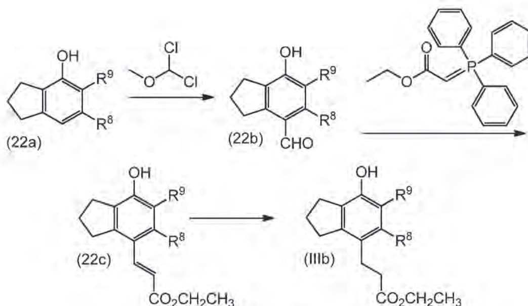
Scheme 20
