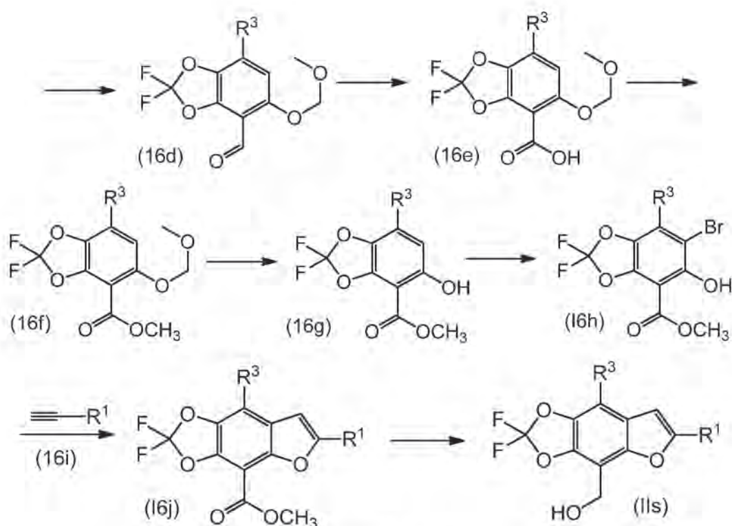
Scheme 16
