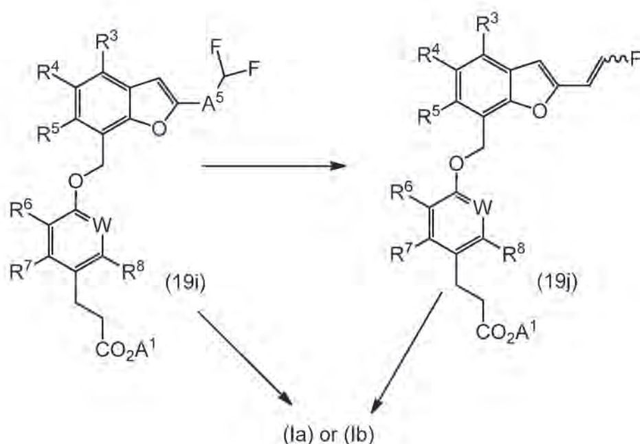
Scheme 20
