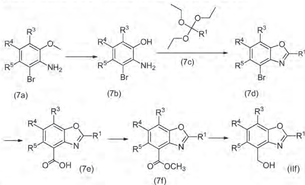
Scheme 7
