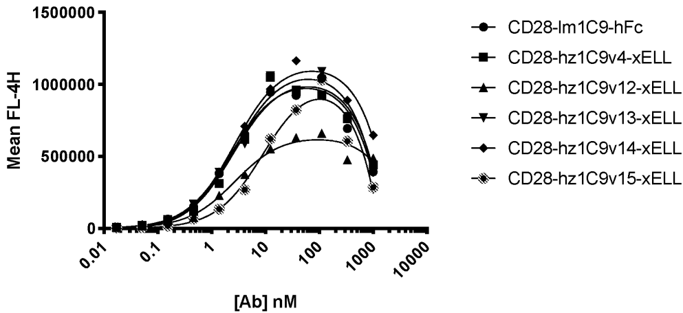
Fig. 2D hCD28-293FS
