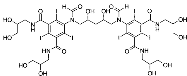
Formula (IIIc)
