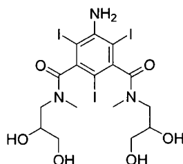
5-Amino-N,N'-bis-(2,3-dihydroxy-propyl)-2,4,6-triiodo-N,N'-dimethyl-isophthalamide
