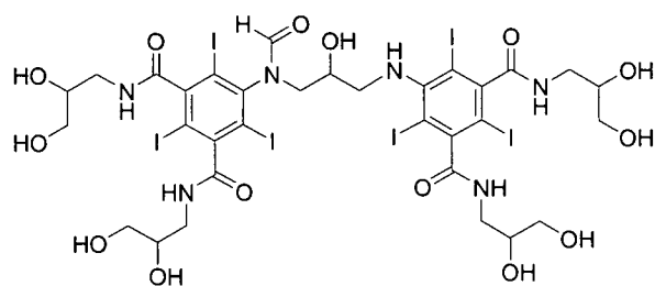
Formula (IIIlu)
