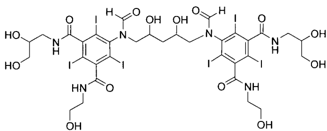
Formula (IIIIm)
