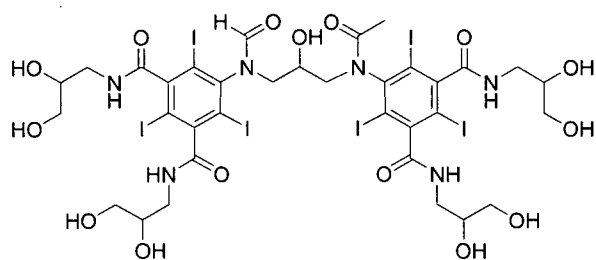
Formula (IIIlt)
