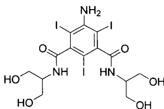
5-Amino-N-(2,3-dihydroxy-propyl)-N'-(2-hydroxy-1-hydroxymethyl-ethyl)-2,4,6-triiodo-isophthalamide (WO2002044125)
