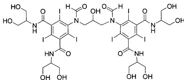
Formula (IIId)
