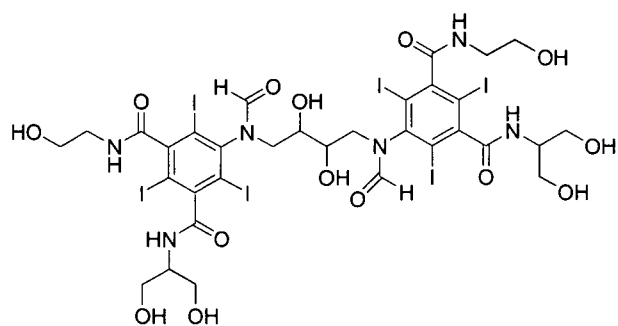
Formula (IIIr)
