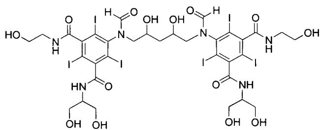
Formula (IIIs)
