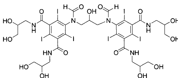
Formula (IIIa)
