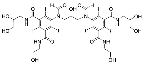
Formula (IIIl)
