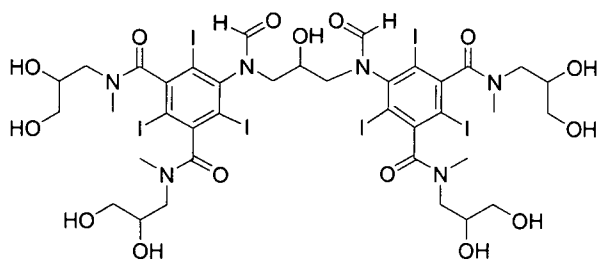
Formula (IIIj)
