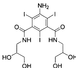
5-Amino-N,N'-bis-(2,3-dihydroxy-propyl)-2,4,6-triiodo-isophthalamide
