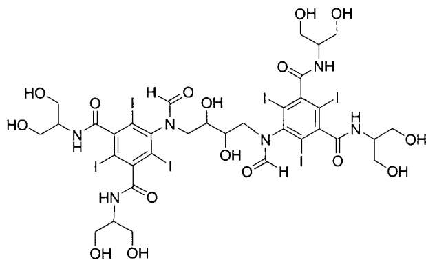
Formula (IIIe)
