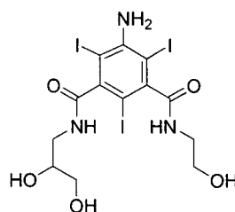
5-Amino-N-(2,3-dihydroxy-propyl)-N'-(2-hydroxy-ethyl)-2,4,6-triiodo-isophthalamide (WO 8700757)
