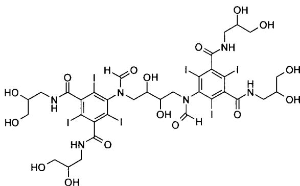
Formula (IIIb)
