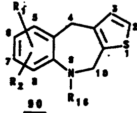
90 (R 16 -H) 4,10-dihydro-9H-thieno[2,3-c][1]benzoxepine
