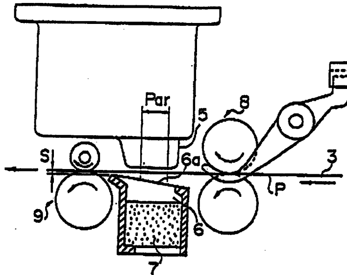
FIG. 18 PRIOR ART
