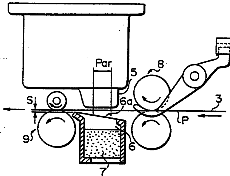
FIG. 17 PRIOR ART
