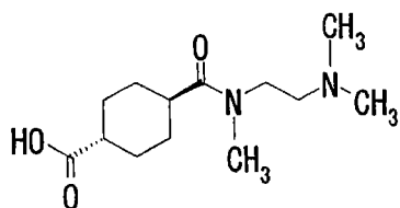
(1) trans-4-(Methoxycarbonyl)cyclohexanecarboxylic acid
