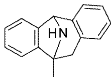
MK801 (dizocilpine)
