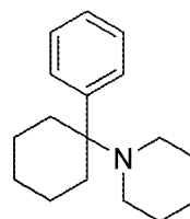
Phencyclidine (PCP)
