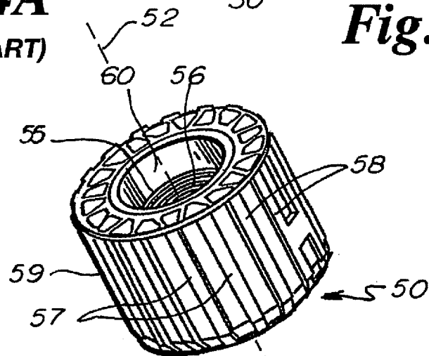
Fig. 4C (PRIOR ART)
