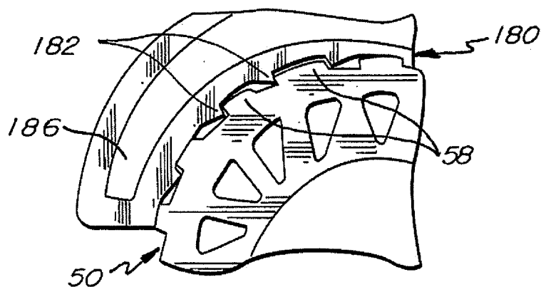
Fig. 5C (PRIOR ART)
