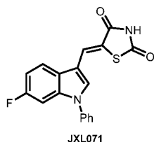
(Z)-5-((6-Fluoro-1-phenyl-1H-indol-3-yl)methylene)thiazolidine-2,4-dione (JXL071)
