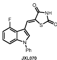
(Z)-5-((4-Fluoro-1-phenyl-1H-indol-3-yl)methylene)thiazolidine-2,4-dione (JXL070)
