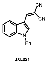
2-((1-Phenyl-1H-indol-3-yl)methylene)malononitrile (JXL021)
