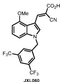
(E)-3-(1-(3,5-Bis(trifluoromethyl)benzyl)-4-methoxy-1H-indol-3-yl)-2-cyanoacrylic acid (JXL060)
