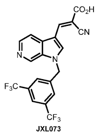
( E )-3-(1-(3,5-Bis(trifluoromethyl)benzyl)-1 H -pyrrolo[2,3- c ]pyridin-3-yl)-2-cyanoacrylic acid (JXL073)
