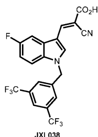
(E)-3-(1-(3,5-Bis(trifluoromethyl)benzyl)-5-fluoro-1H-indol-3-yl)-2-cyanoacrylic acid (JXL038)
