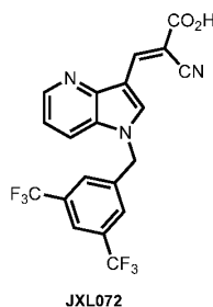
(E)-3-(1-(3,5-Bis(trifluoromethyl)benzyl)-1H-pyrrolo[3,2-b]pyridin-3-yl)-2-cyanoacrylic acid (JXL072)
