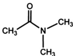
N,N-dimethylacetamide
