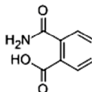
Phthalamic acid
