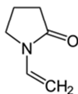
N-vinyl-2-pyrrolidone
