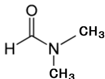
N,N-dimethylformamide
