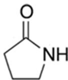
2-Pyrrolidone
