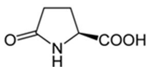
L-pyrroglutamic acid
