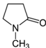
N-methyl-2-pyrrolidone
