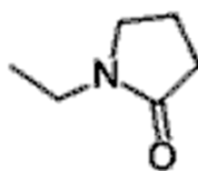
1-Ethyl-2-pyrrolidone
