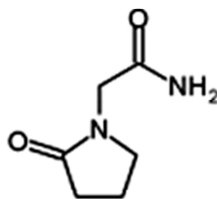
Piracetam
