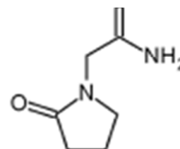
Piracetam
