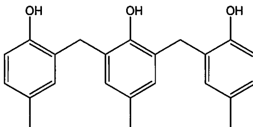
2,2'-((2-hydroxy-5-methyl-1,3-phenylene)bis(methylene))bis(4-methylphenol)
