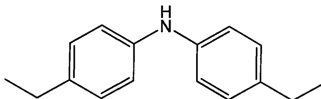
bis(4-ethylphenyl)amine
