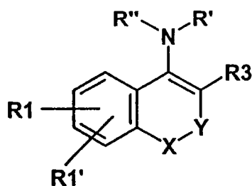
Formula XIII
