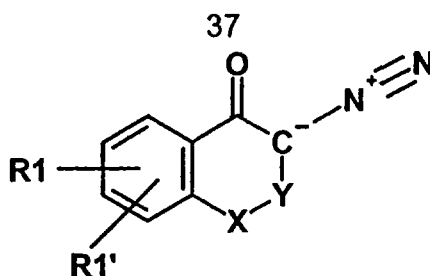
Formula VIII
