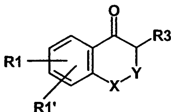
Formula X
