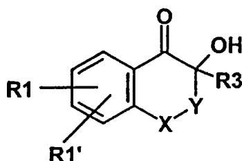
Formula XI
