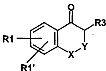
Formula X
