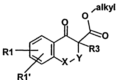
Formula XIV
