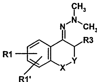
Formula XII
