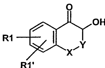
Formula IX.
