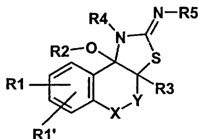
Formula I
