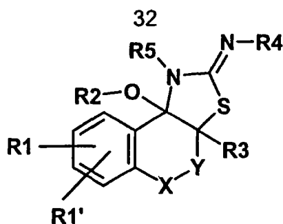
Formula Ib.
