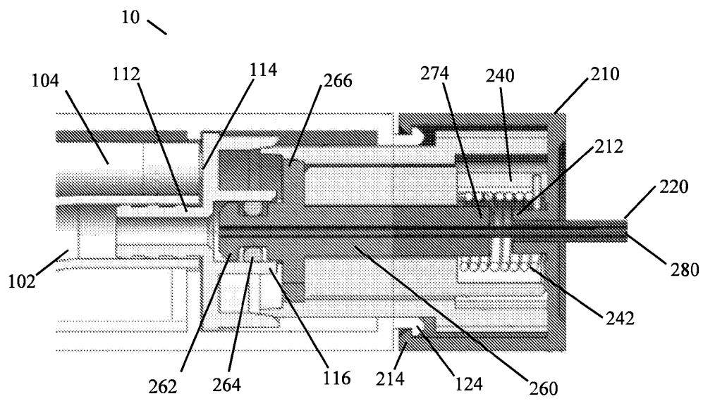
Figure 2B Section A-A
