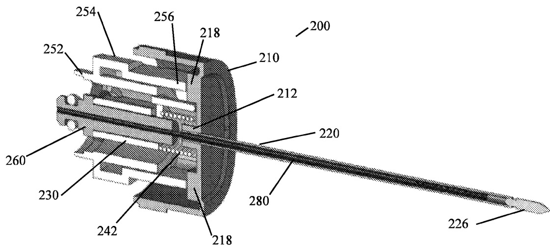
Figure 5B Section B-B
