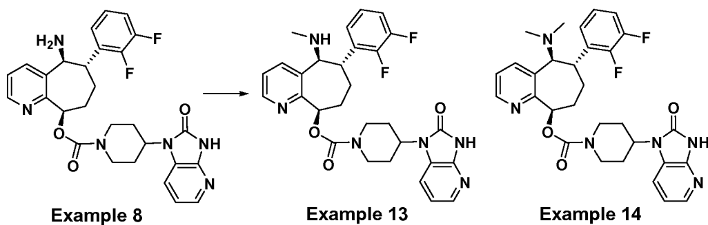
Scheme 7:
