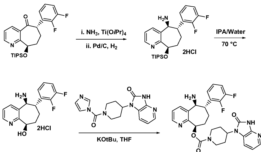
Scheme 3a:
