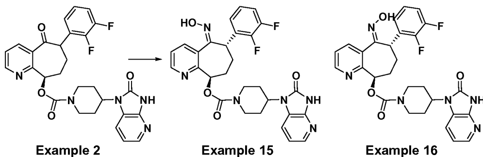
Scheme 8:
