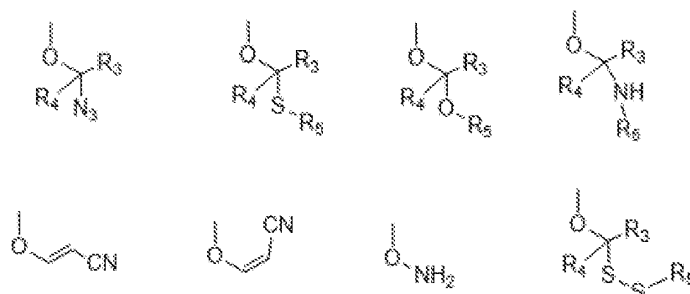
Structures VI-XIII
