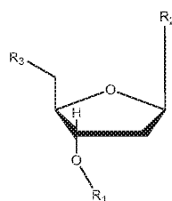
Structure I
