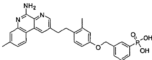
Scheme 4
