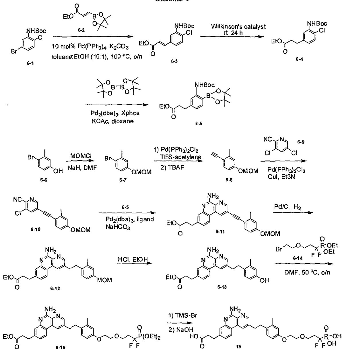
Scheme 6
