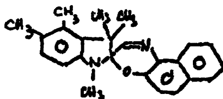
1,3,3,5,6-pentamethylspiro(indolino-2,3'-[3H]naphtho(2,1b)-(1,4)oxazine)
