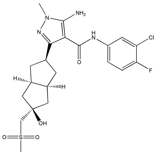
Fig. 2 The relative stereochemistry scheme of compound AIA-227-2.
