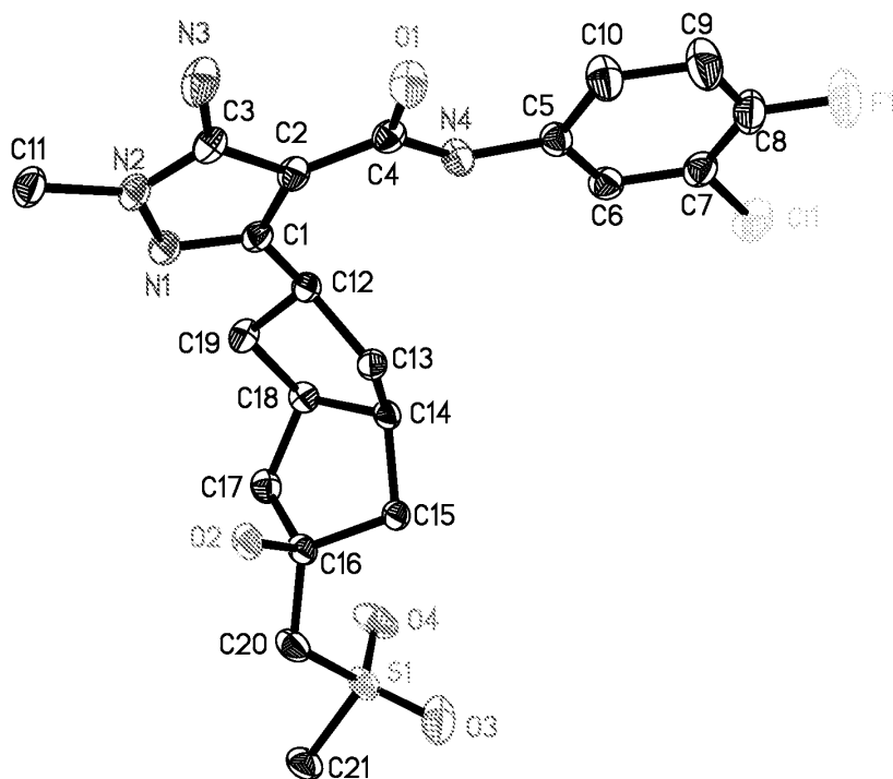
Fig. 1 The ORTEP plot for compound AIA-227-2
