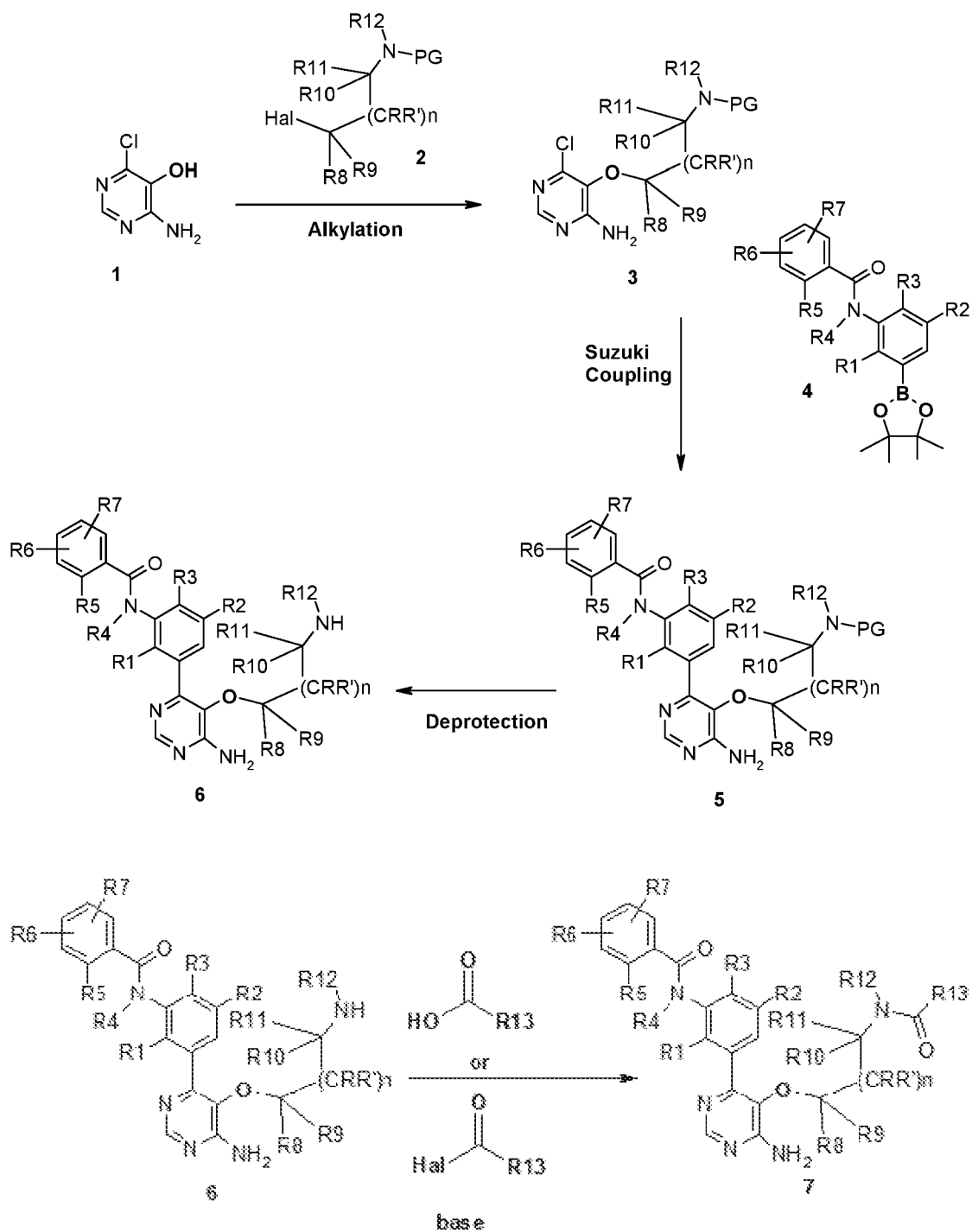
Scheme 1:
