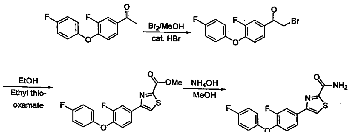
Scheme 8
