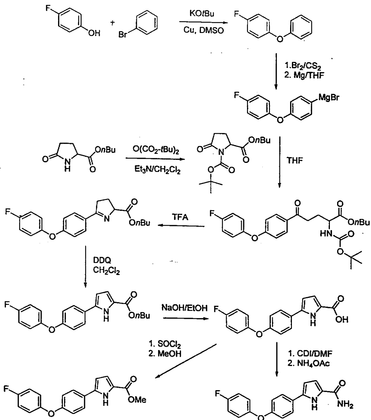
Scheme 6
