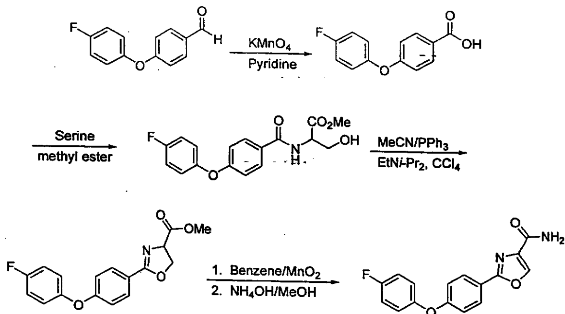
Scheme 7
