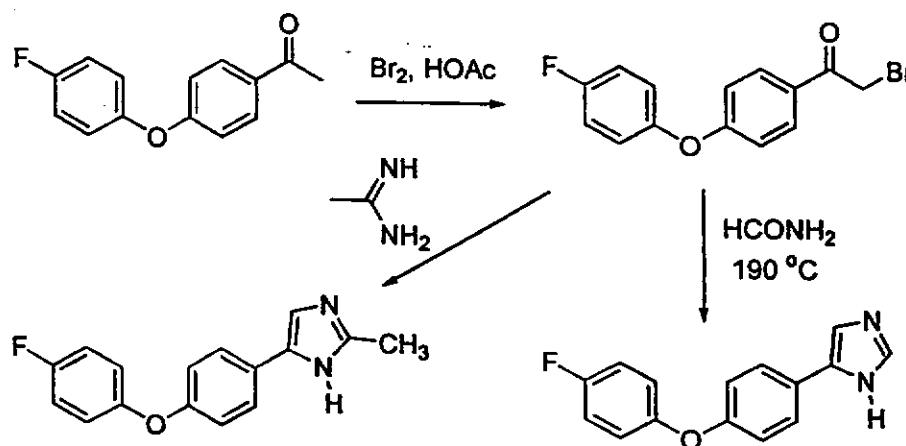
Scheme 5
