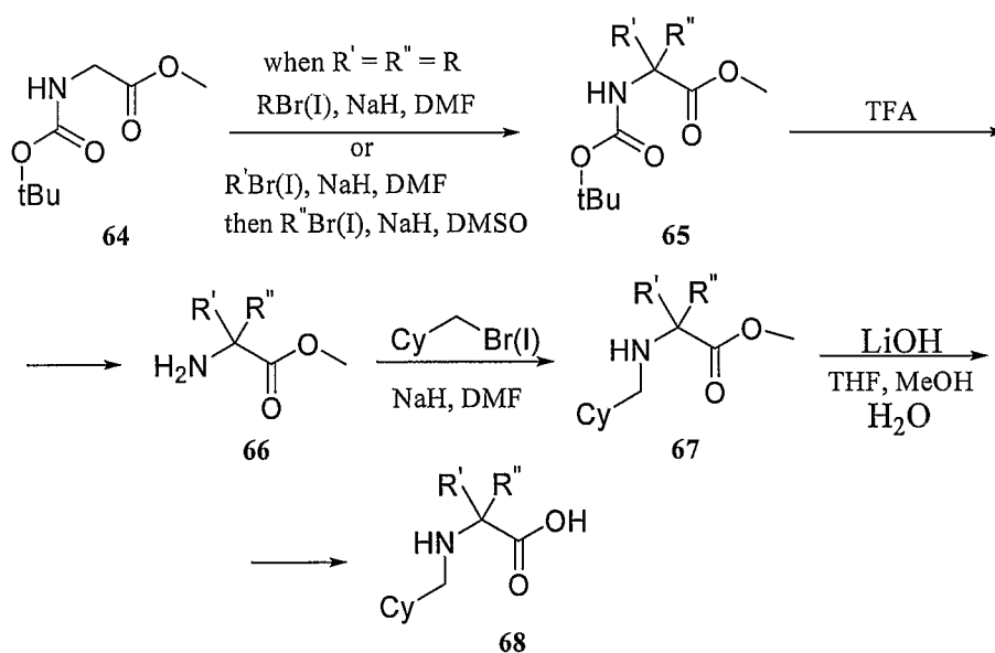
Scheme 18
