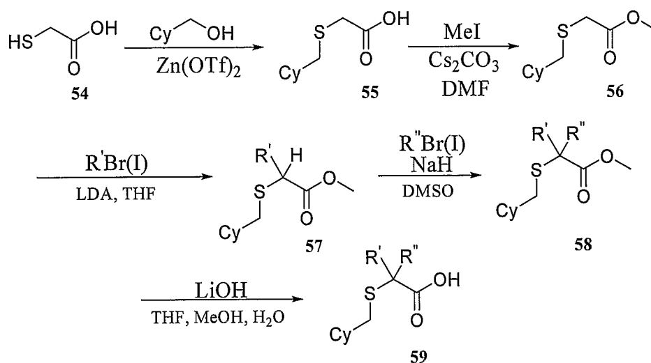
Scheme 16
