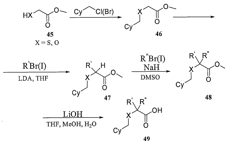
Scheme 14
