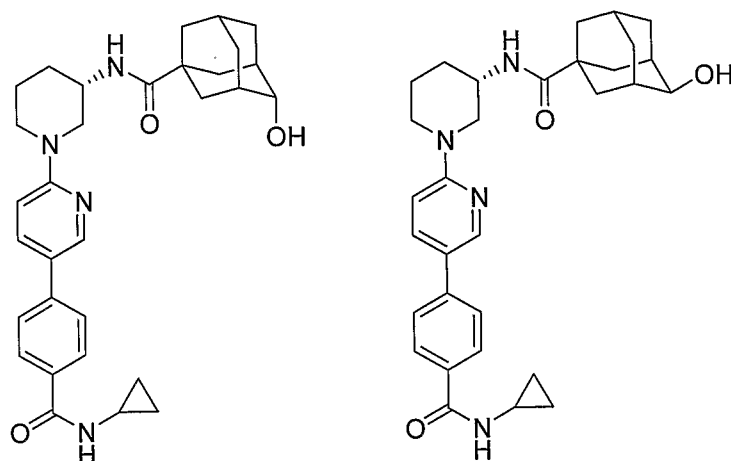
N-[(3S)-1-(5-{4-[(Cyclopropylamino)carbonyl]phenyl}pyridin-2-yl)piperidin-3-yl]-4-hydroxyadamantane-1-carboxamide
