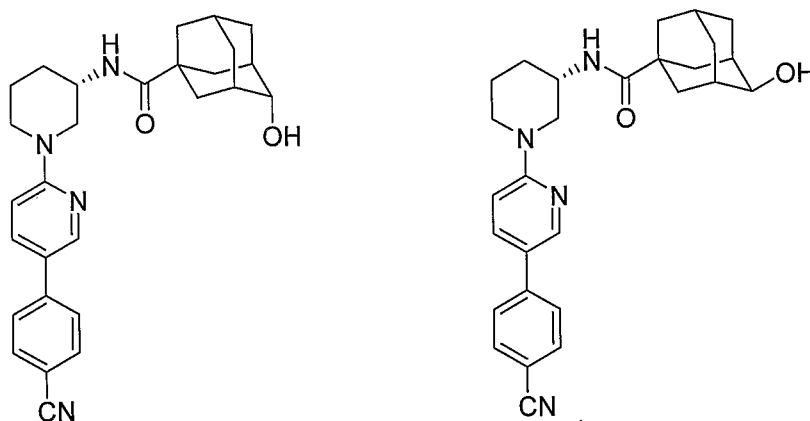
N-{(3S)-1-[5-(4-cyanophenyl)pyridin-2-yl]piperidin-3-yl}-4-hydroxyadamantane-1-carboxamide
