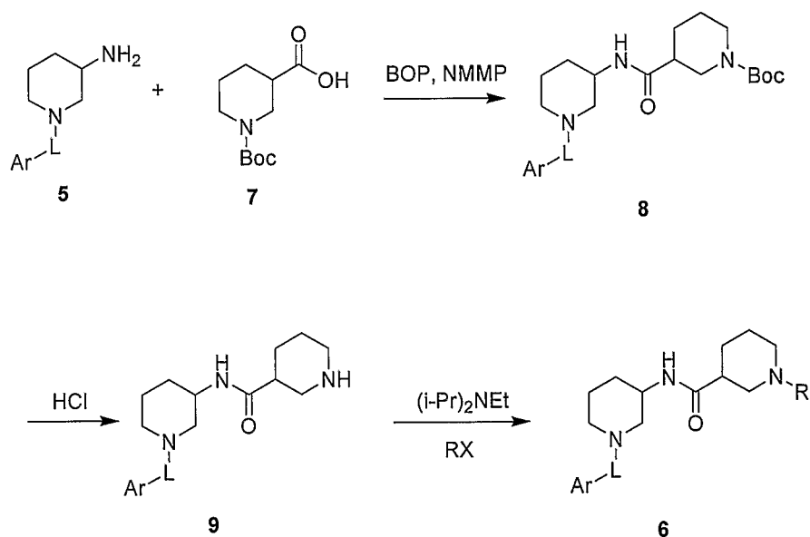
Scheme 4
