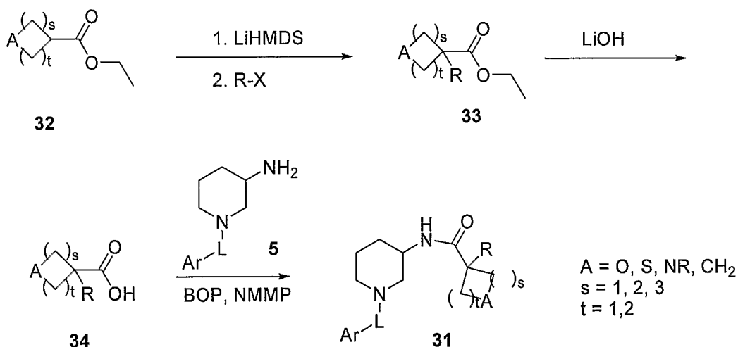
Scheme 10
