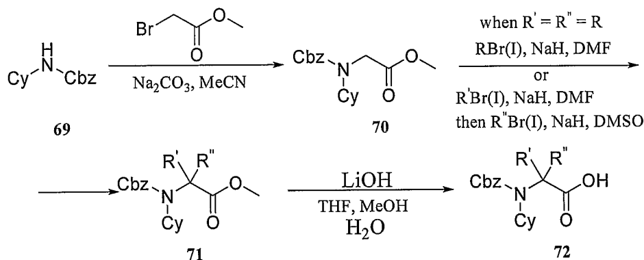
Scheme 20
