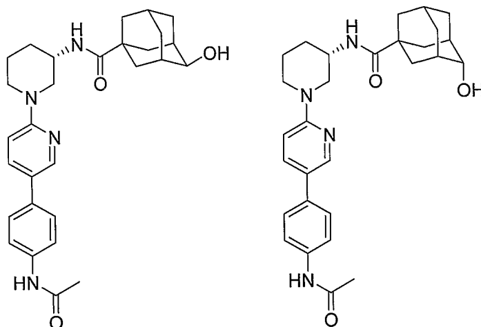
N-((3S)-1-{5-[4-(Acetylamino)phenyl]pyridin-2-yl}piperidin-3-yl)-4-hydroxyadamantane-1-carboxamide
