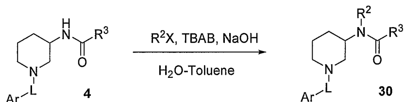
Scheme 9
