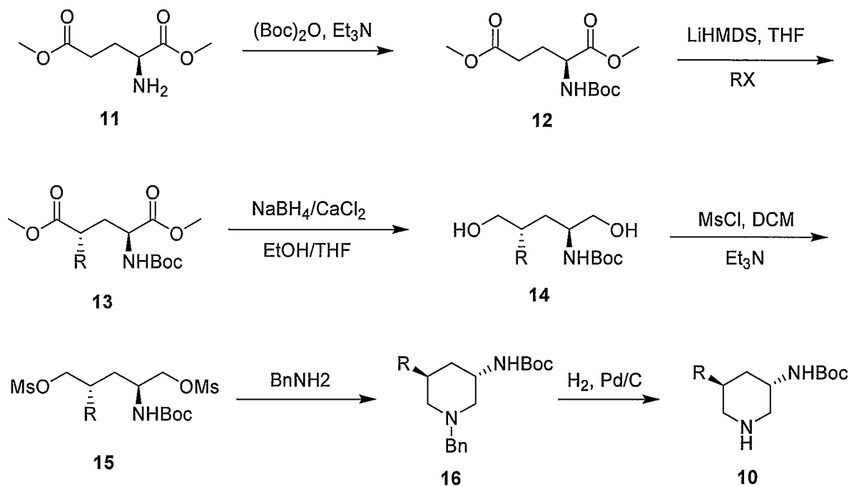
Scheme 5
