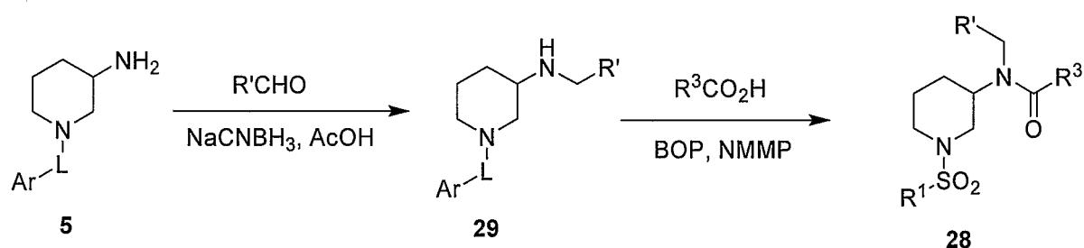
Scheme 8
