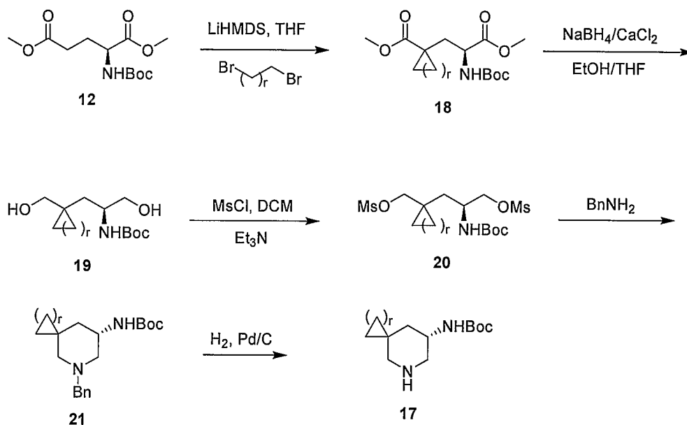
Scheme 6
