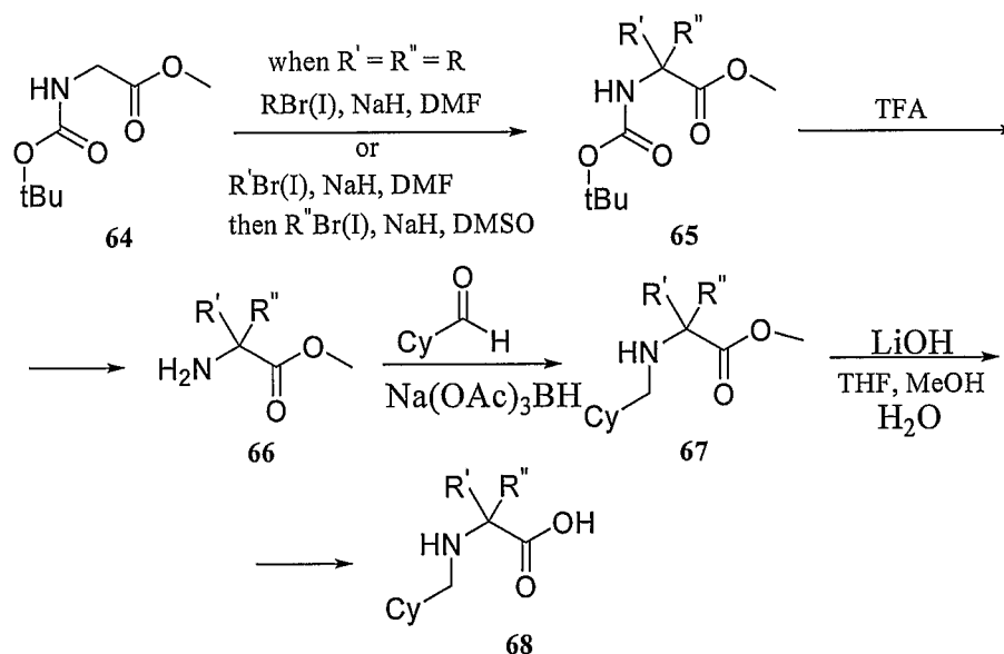
Scheme 19
