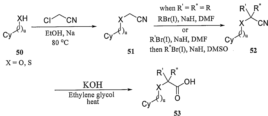
Scheme 15
