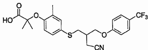
Compound 18
