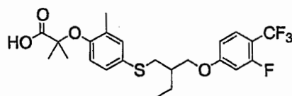
Compound 7
