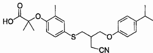
Compound 13
