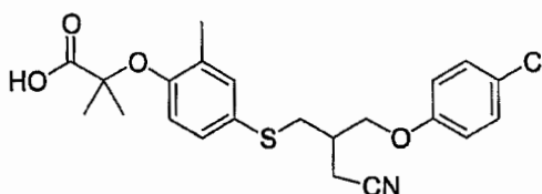
Compound 15
