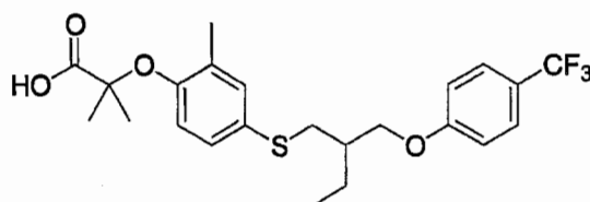
compound 4 #26171158#
