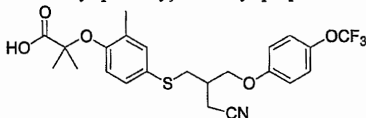
Compound 14
