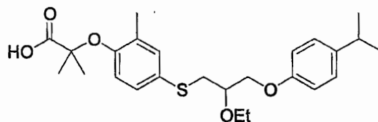
Compound 8
