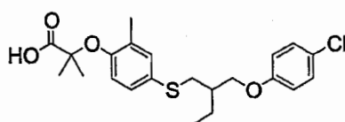
Compound 5
