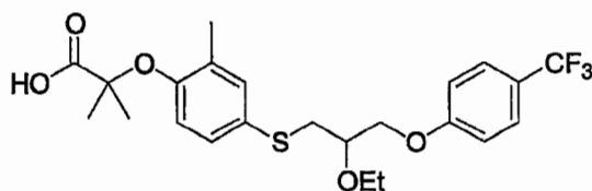
Compound 3
