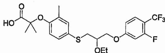
Compound 12
