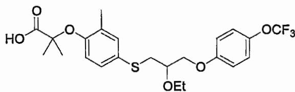
Compound 9
