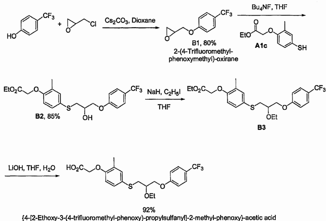
Scheme B
