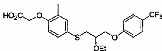
{4-[2-Ethoxy-3-(4-trifluoromethyl-phenoxy)-propylsulfanyl]-2-methyl-phenoxy}-acetic acid
