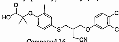
Compound 16
