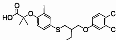
Compound 6
