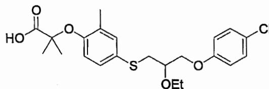
Compound 10
