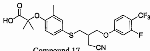
Compound 17
