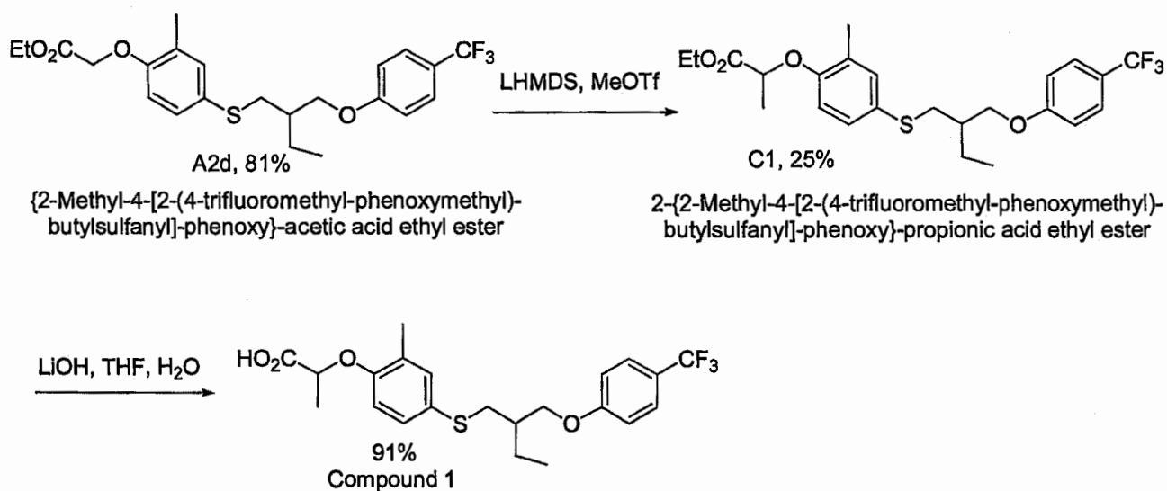
Scheme C
