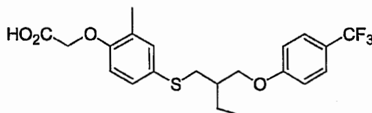
{2-Methyl-4-[2-(4-trifluoromethyl-phenoxy)methyl]-butylsulfanyl]-phenoxy}-acetic acid
