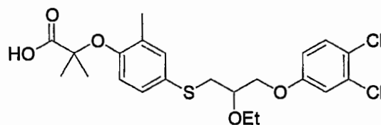
Compound 11
