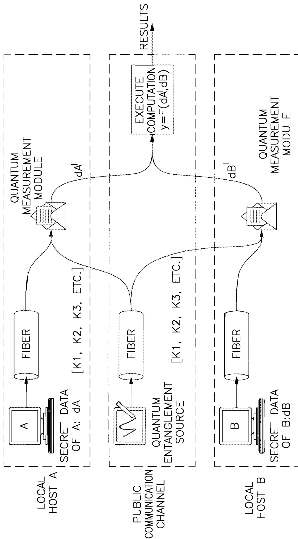
SYSTEM LEVEL DIAGRAM OF QTP2C FOR TWO PARTIES
