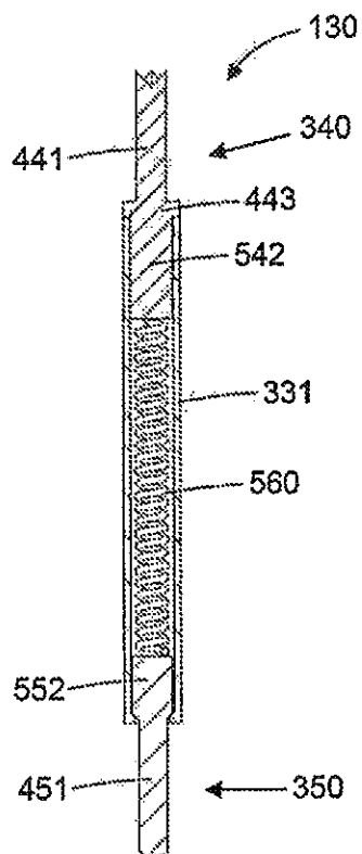
FIG. 5 PRIOR ART
