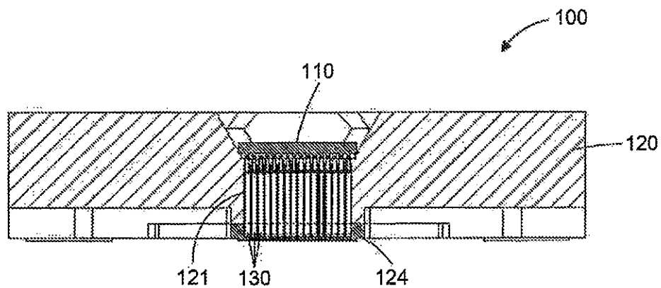
FIG. 1 PRIOR ART
