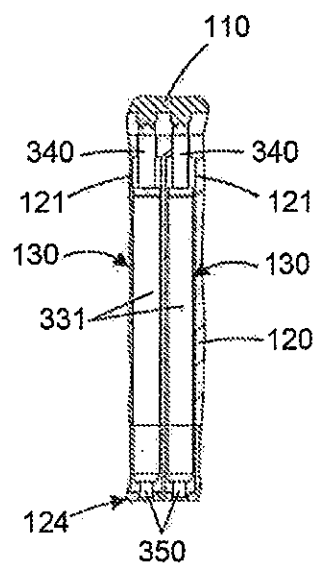
FIG. 3 PRIOR ART
