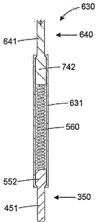
FIG. 7 PRIOR ART
