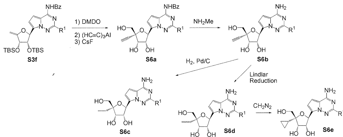
Scheme 6.
