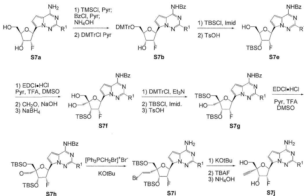
Scheme 7.
