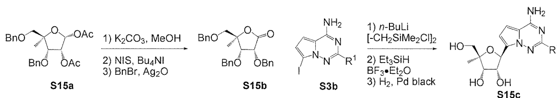
Scheme 15.
