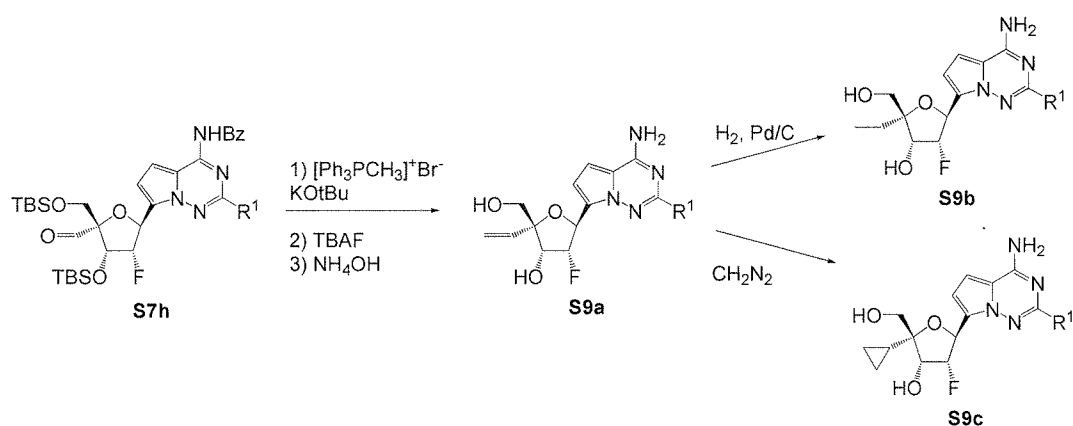
Scheme 9.
