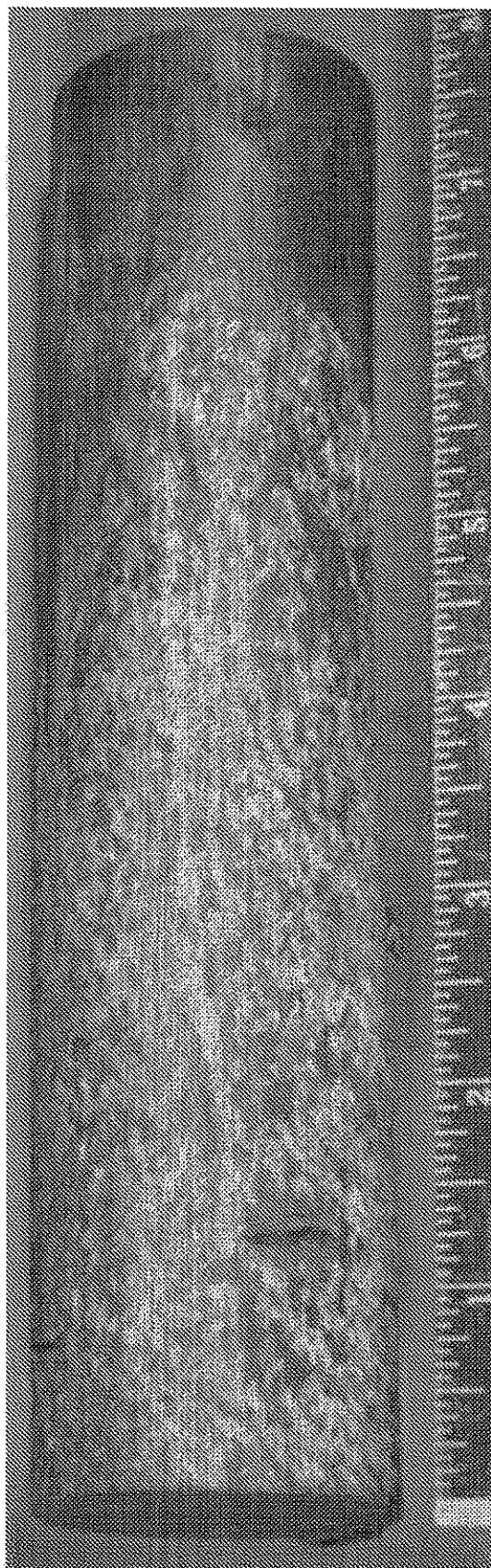
IN 718 <111> Single Crystal Extruded 4:1
