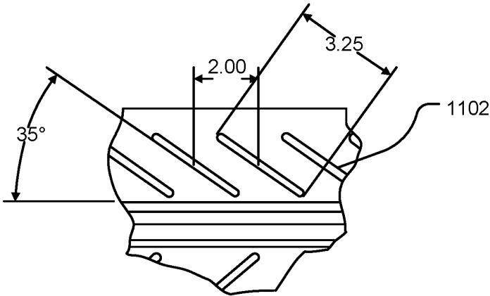
DETAIL B
