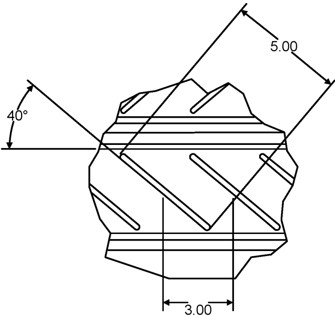
DETAIL A
