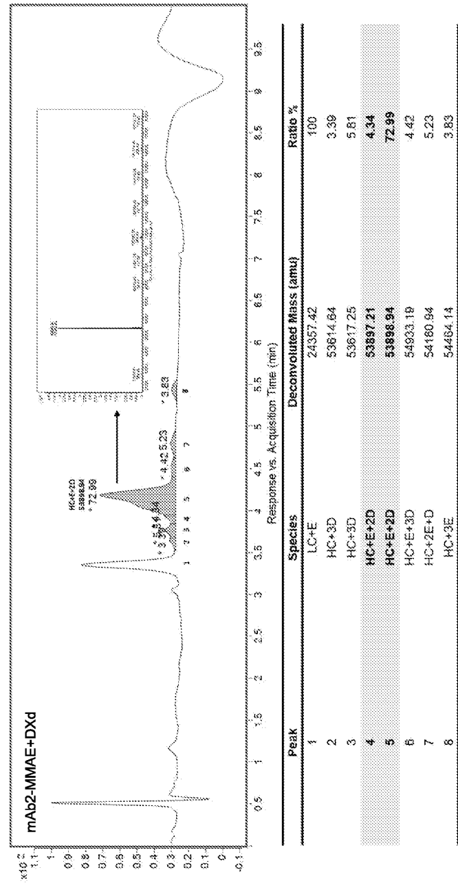
LC stands for Light chain abbreviation; HC stands for Heavy chain abbreviation; E stands for MMAE abbreviation; D stands for DXd abbreviation
