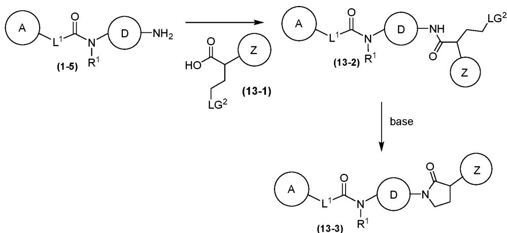
Scheme 13: Representative scheme for synthesis of exemplary compounds of the invention.
