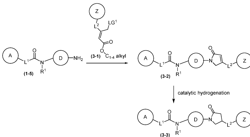
Scheme 3: Representative scheme for synthesis of exemplary compounds of the invention.
