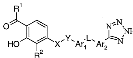
tautomer II
