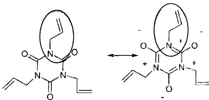
Formula 1 1,3,5-Triallyl-1,3,5-triazine-2,4,6 (1H,3H,5H)trione and the tautomeric form
