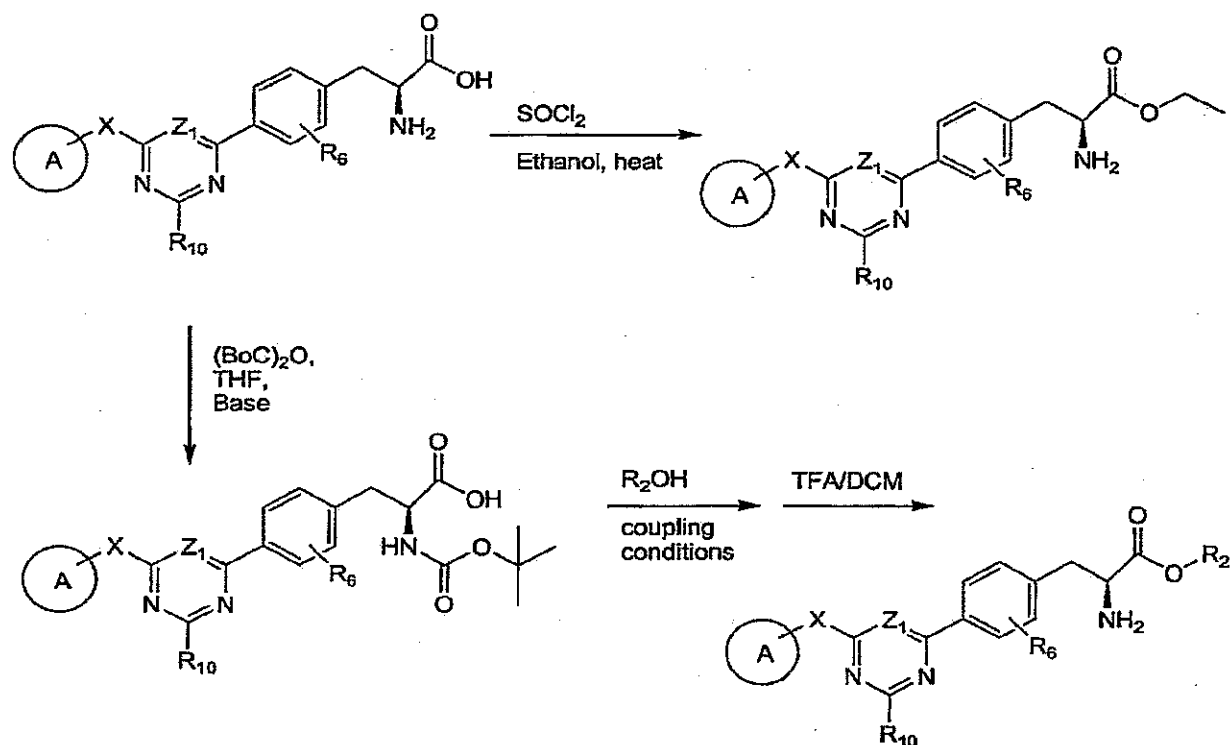
Scheme 5
