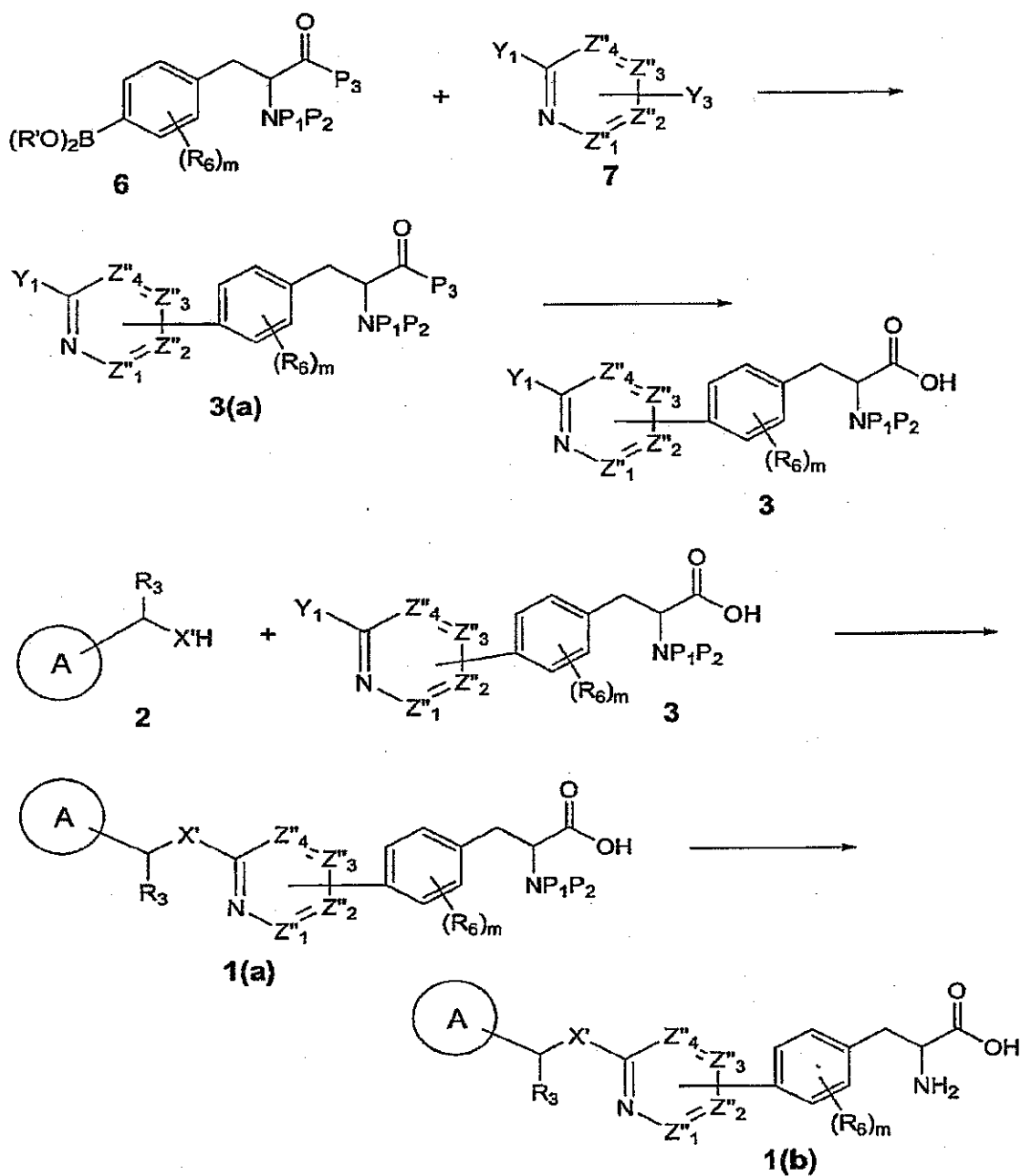
Scheme 3
