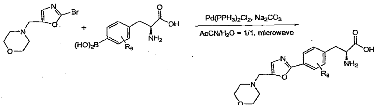
Scheme 7
