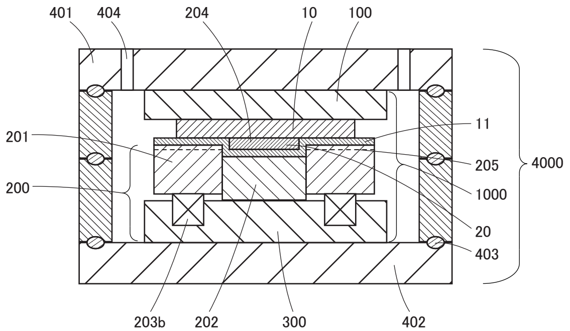
Cross-sectional view B-B
