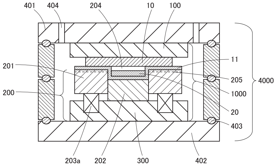
Cross-sectional view A-A
