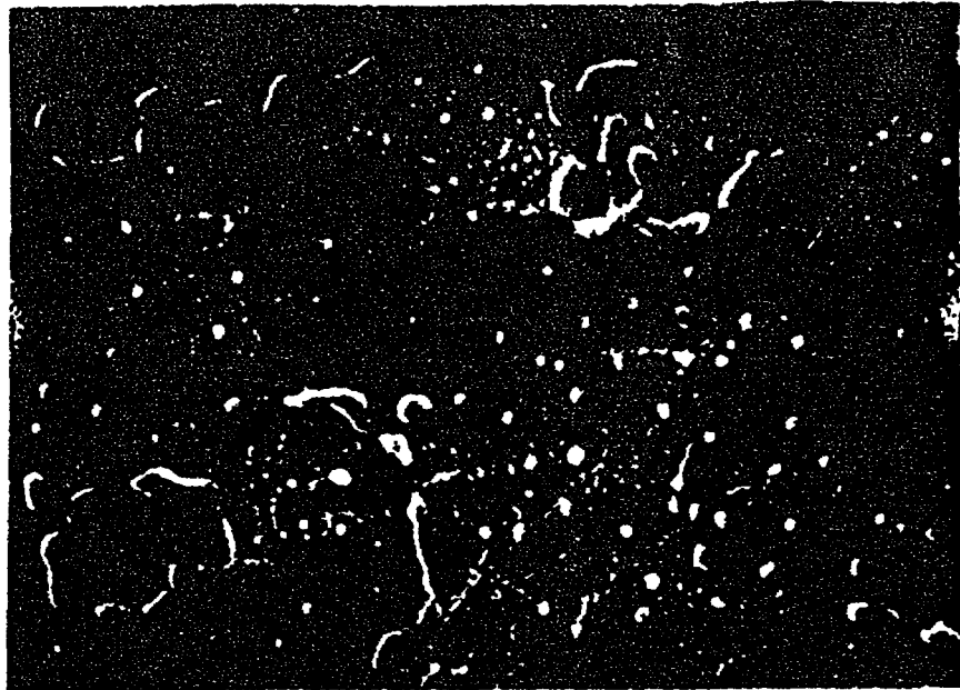
Figure 3 shows a SEM photo of Alloy 1983B annealed at 1800 deg. F, containing approximately ten percent Chi phase. Original magnification 2500X (SR92:0058).
