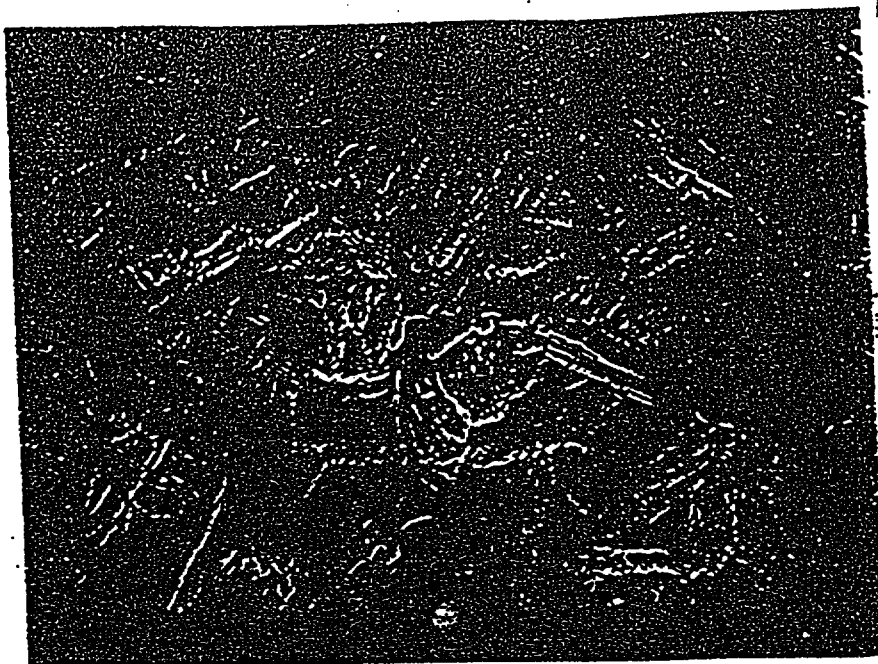
Figure 1 shows a SEM photo of Alloy 105A annealed at 2000 deg. F, showing the martensitic microstructure. Original magnification 500X (SR92:0792).
