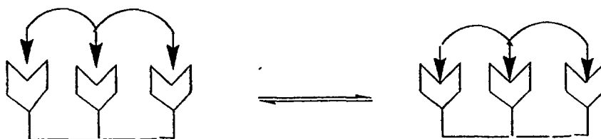
trivalent interaction
