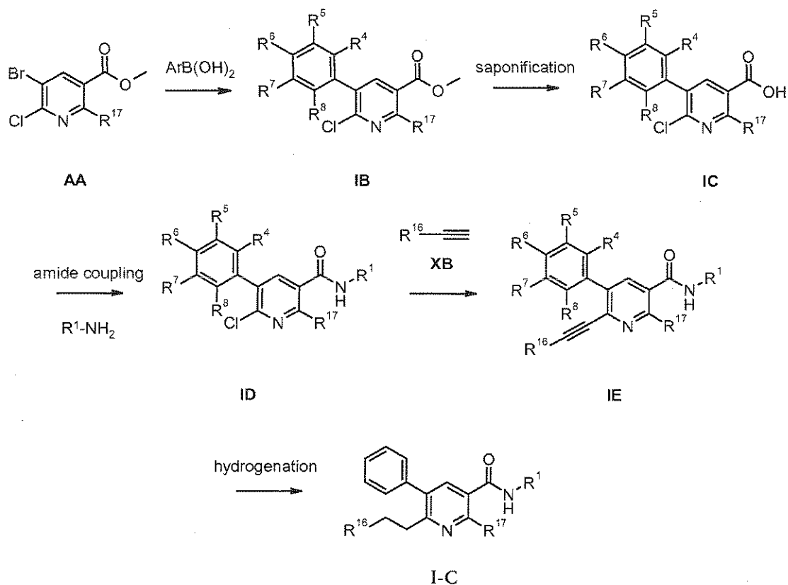
Scheme 9
