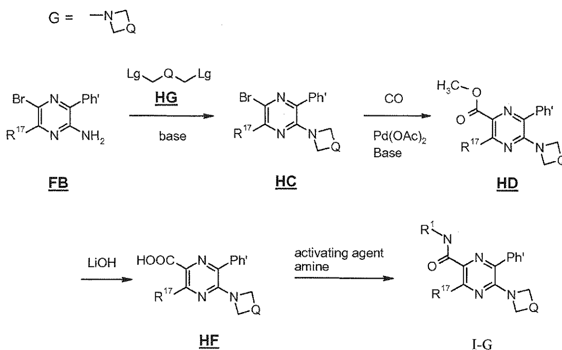
Scheme 8
