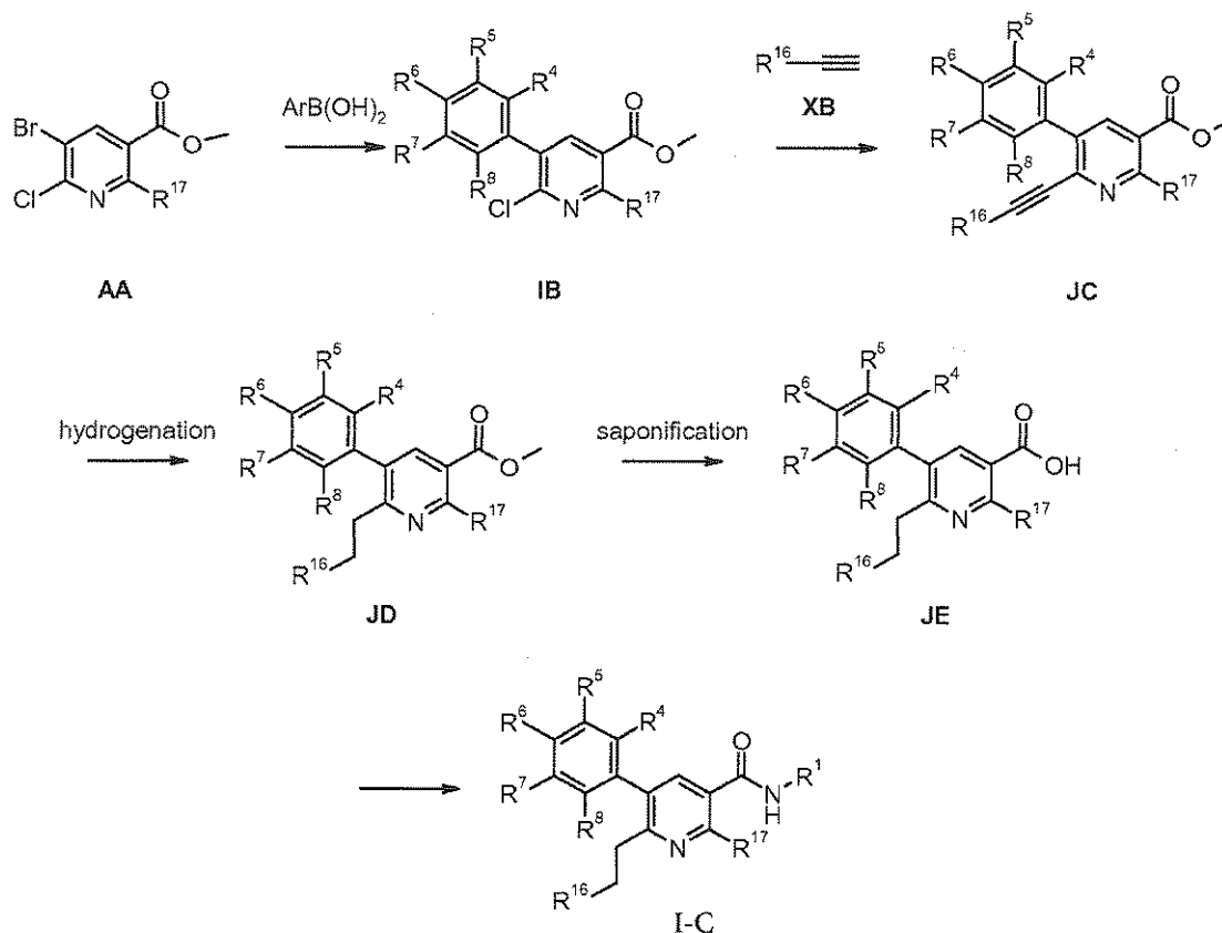
Scheme 10
