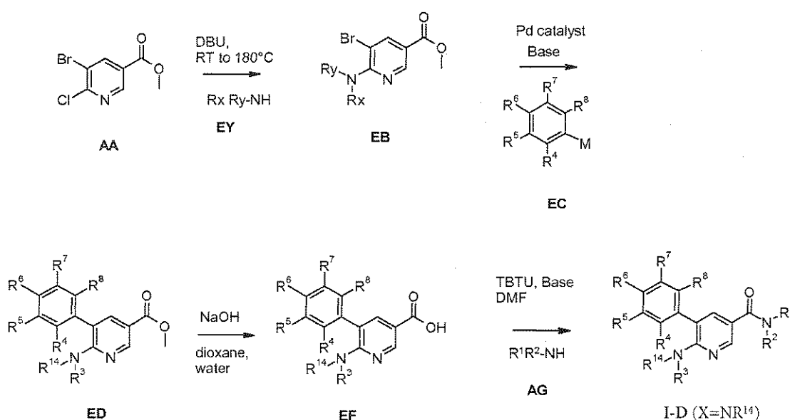
Scheme 5
