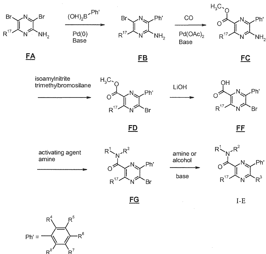
Scheme 6
