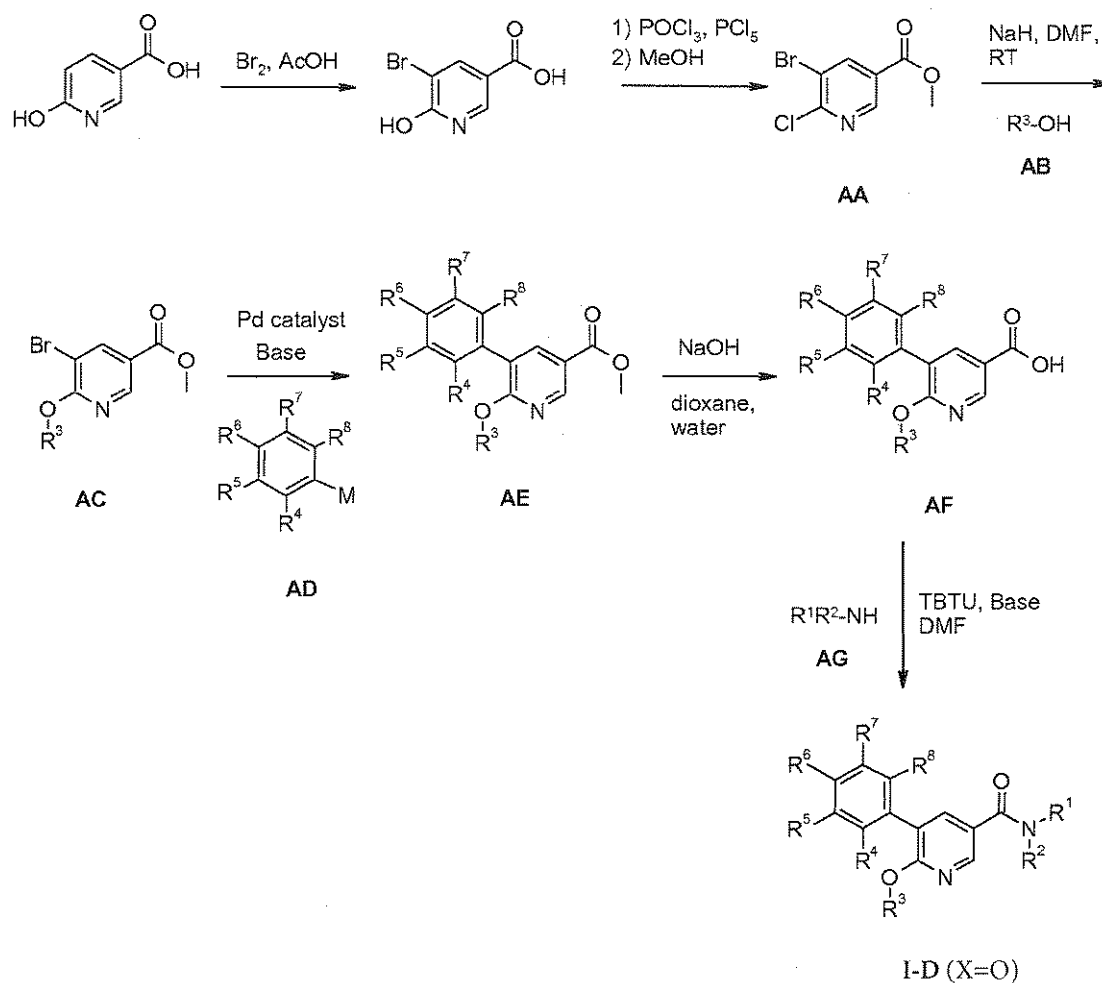
Scheme 1
