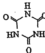
Cyanuric acid
