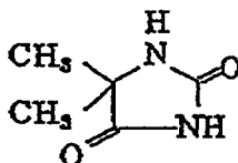
3-Methyl-5-pyrazolone
