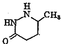
6-Methyl-3-pyridazone
