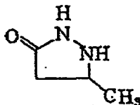
3-Methyl-5-pyrazolone
