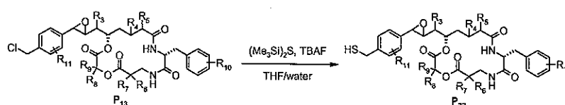
Scheme 6
