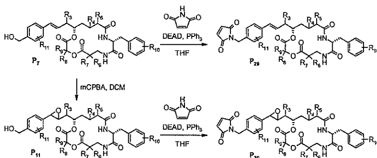
Scheme 8
