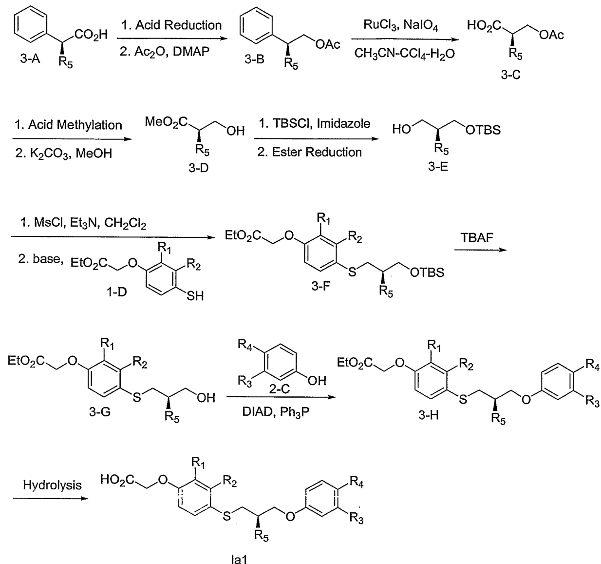
Scheme 3. Synthesis of Compound Ia1
