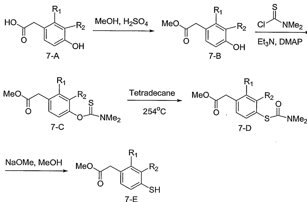
Scheme 7. Synthesis of Intermediate 7-E
