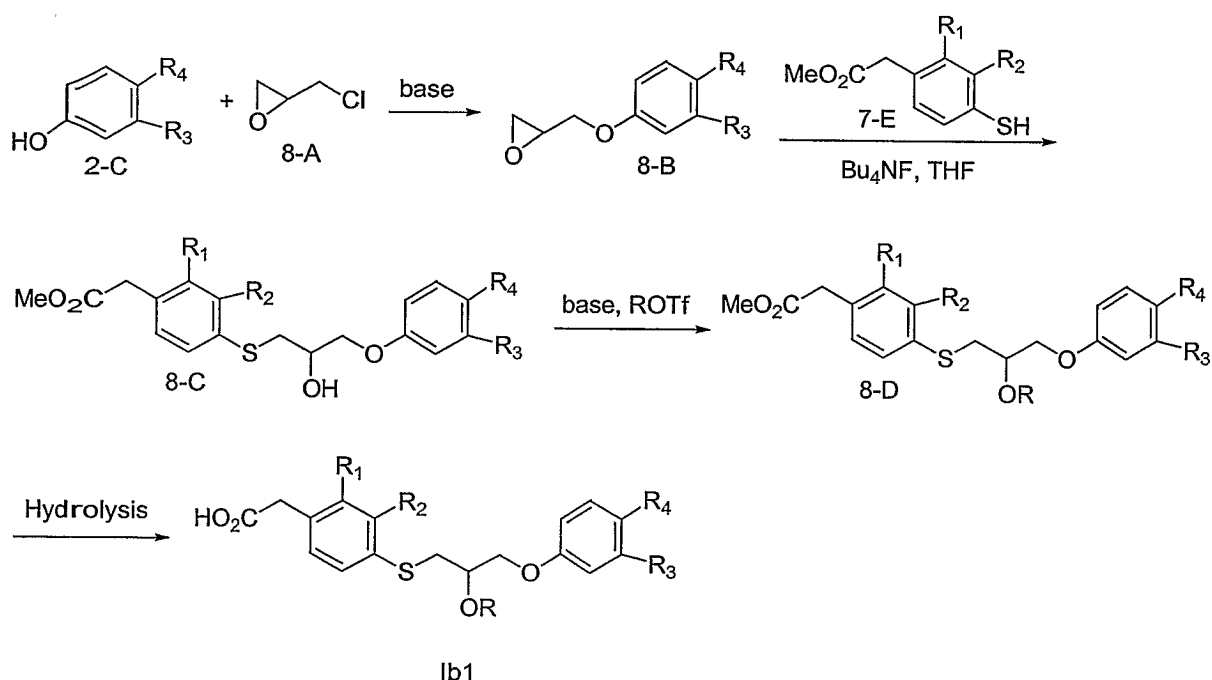
Scheme 8. Synthesis of Compound Ib1
