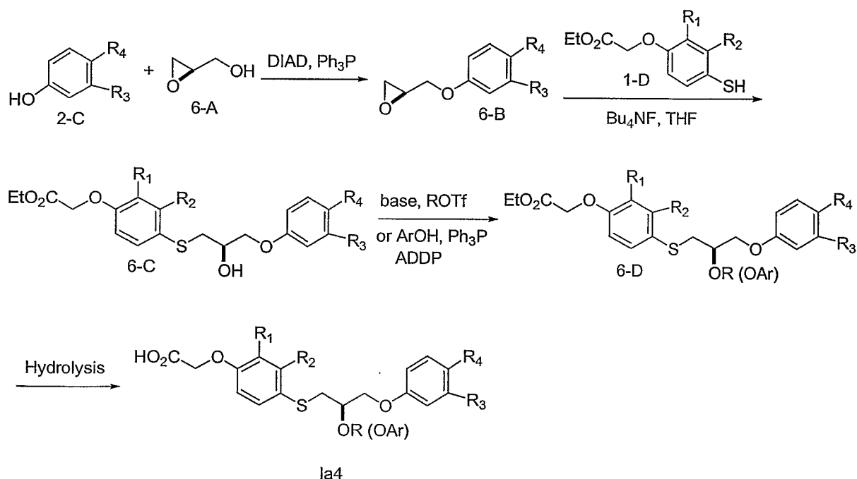
Scheme 6. Synthesis of Compound 1a4
