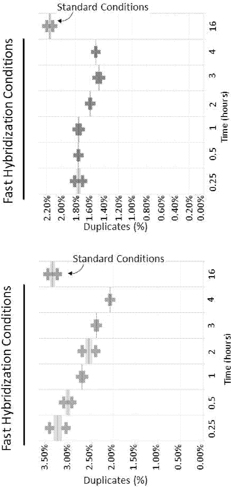
33.1 Mb Exome 0.8 Mb Custom Panel FIG. 37E
