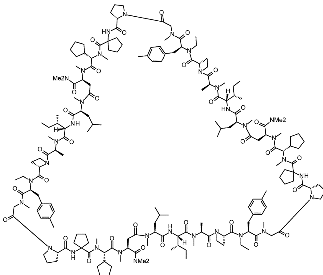
b7 (Cyclic Trimer)
