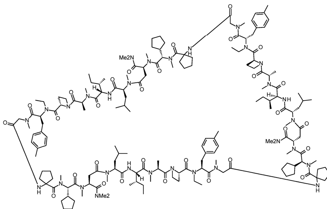
c8 (Cyclic Trimer)
