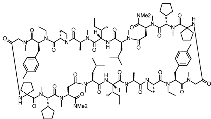
c7 (Cyclic Dimer)
