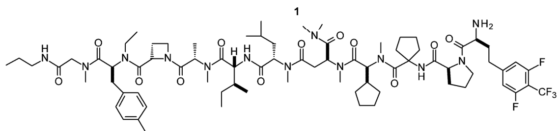
Propylamide of Compound 35
