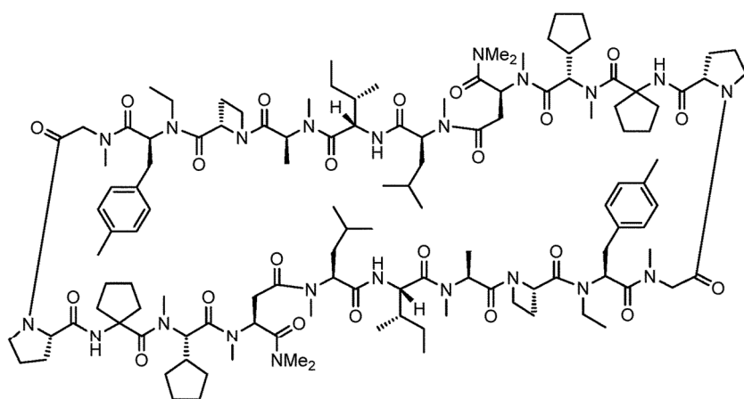
b6 (Cyclic Dimer)
